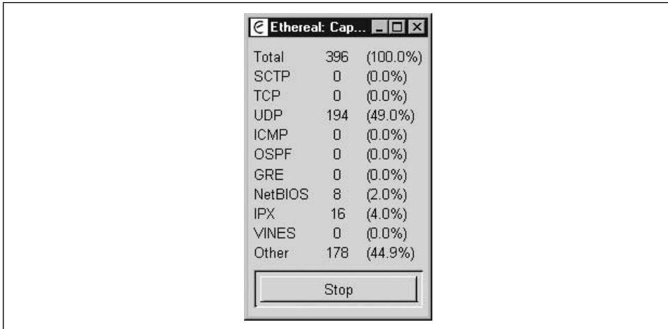
Figure 5-3. ethereal Capture
