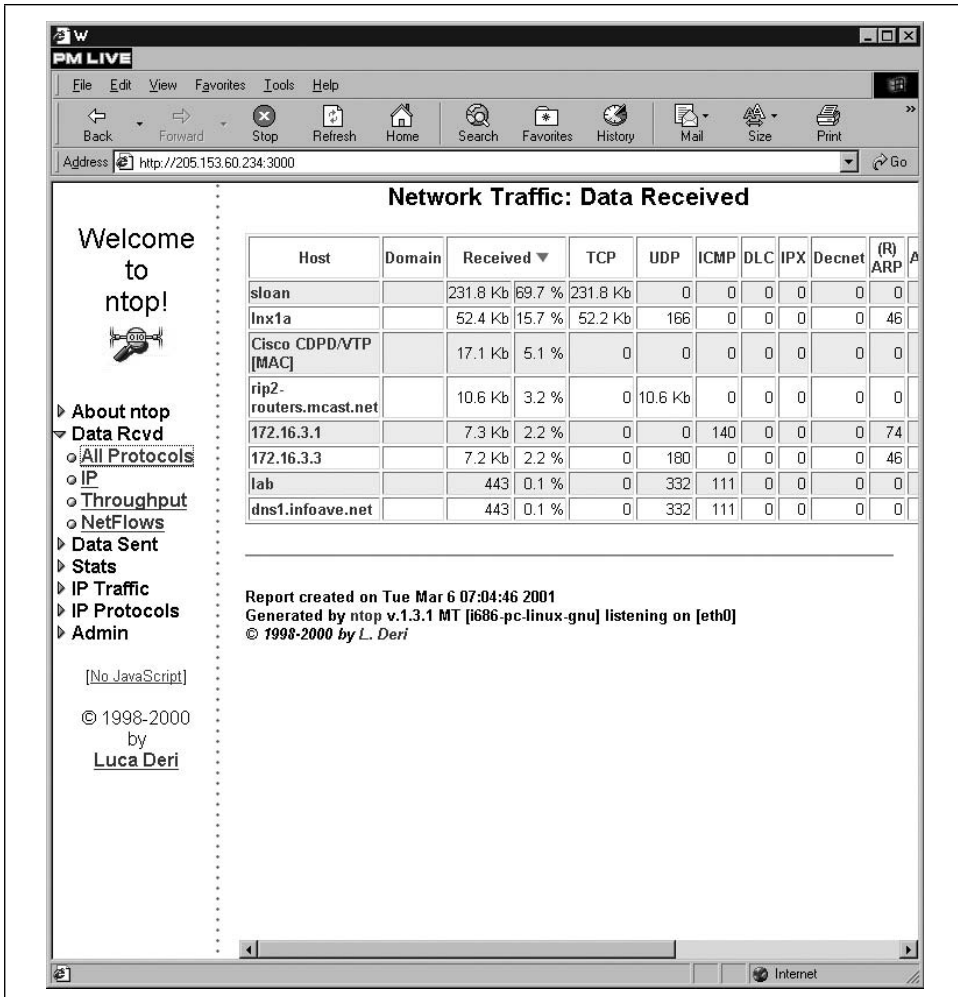
Figure 8-2. ntop's All Protocols page
