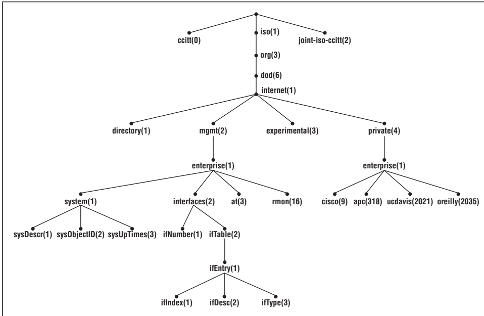
Figure 7-2. Partial OID structure
