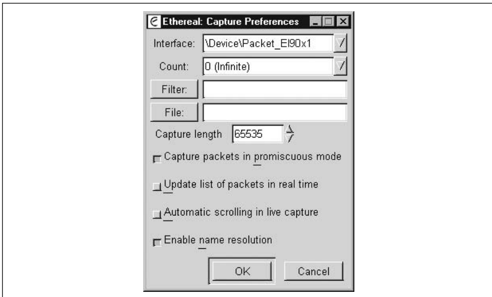
Figure 5-2. ethereal Capture Preferences
