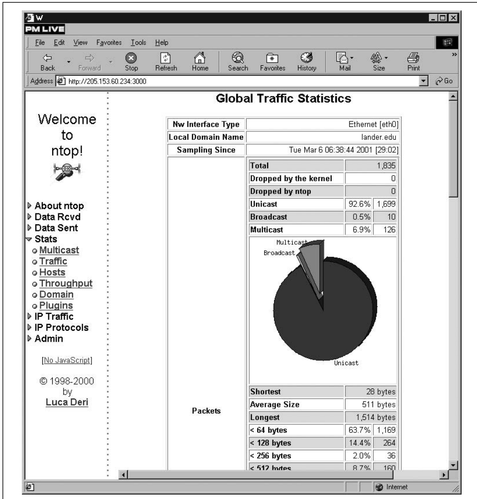
Figure 8-3. ntop's Traffic page under Stats
