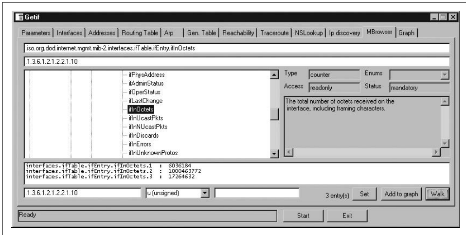
Figure 7-15. getif MBrowser tab
