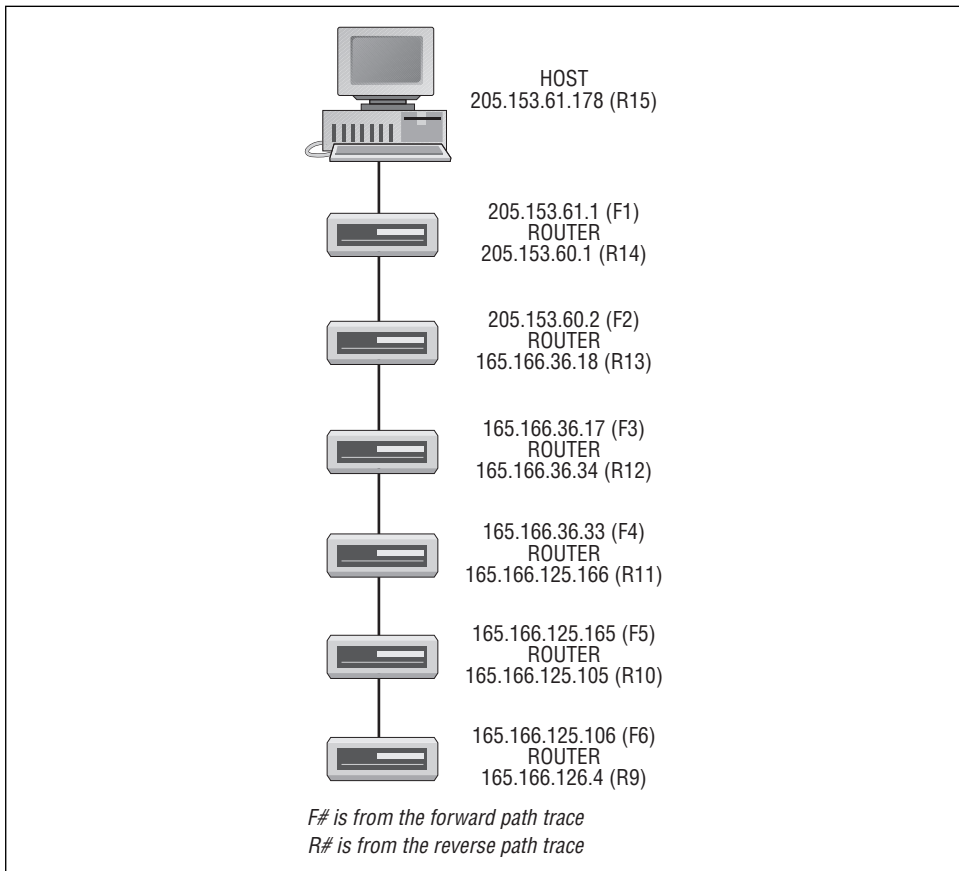
Figure 4-1. First six hops on path
