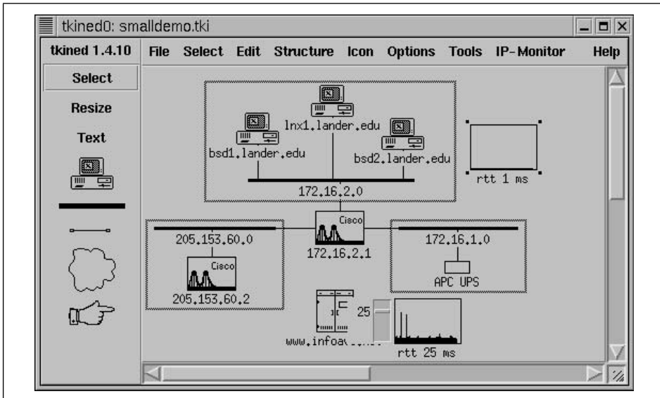
Figure 7-6. Map with stripcharts
