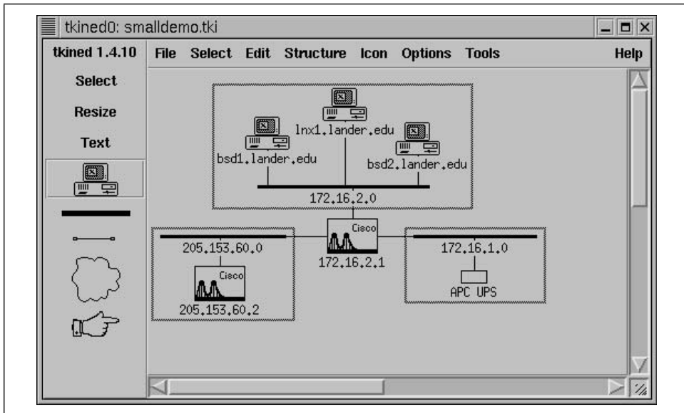
Figure 7-3. Demo network
