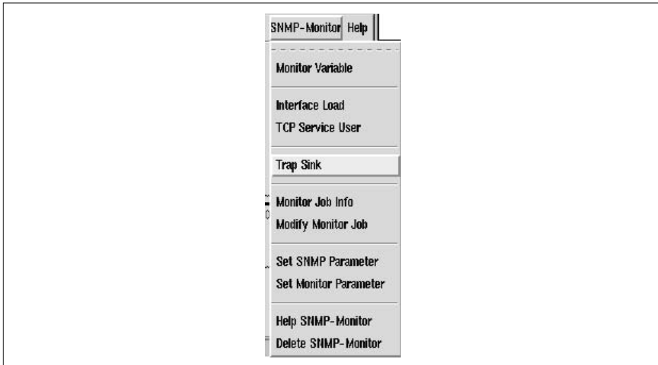
Figure 7-7. SNMP-Monitor menu
