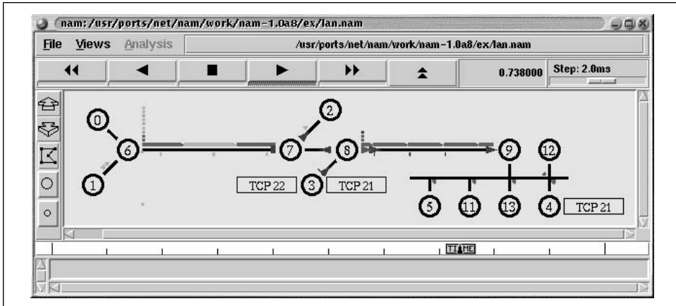
Figure 9-1. nam example
