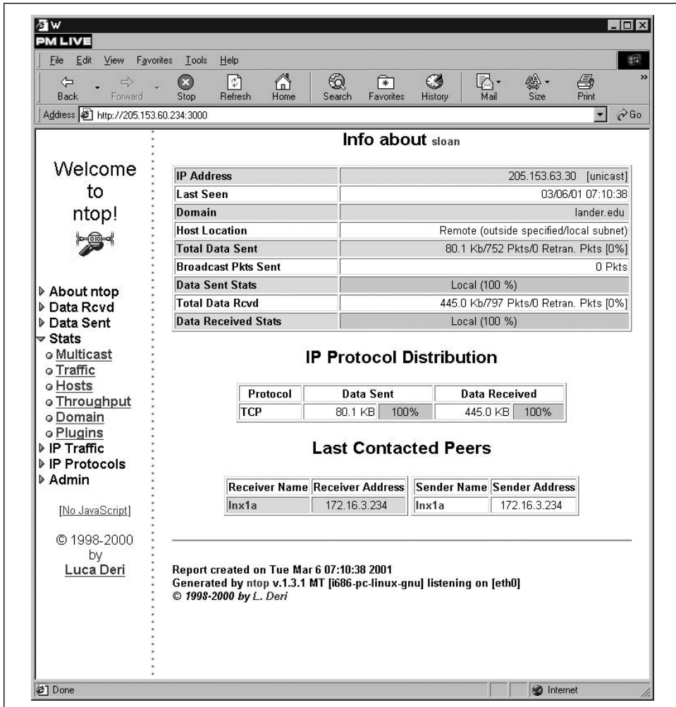
Figure 8-4. Host information
