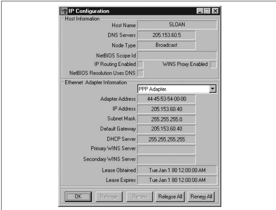
Figure 2-2. winipcfg
