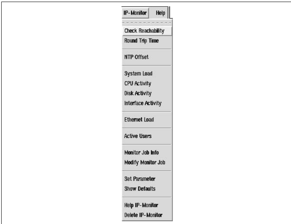
Figure 7-4. IP-Monitor menu
