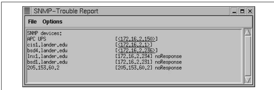
Figure 7-12. SNMP devices
