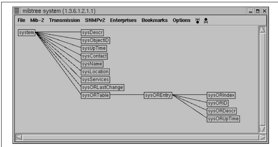
Figure 7-9. SNMP tree
