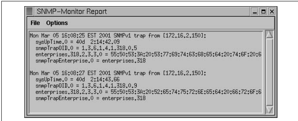
Figure 7-8. SNMP monitor report
