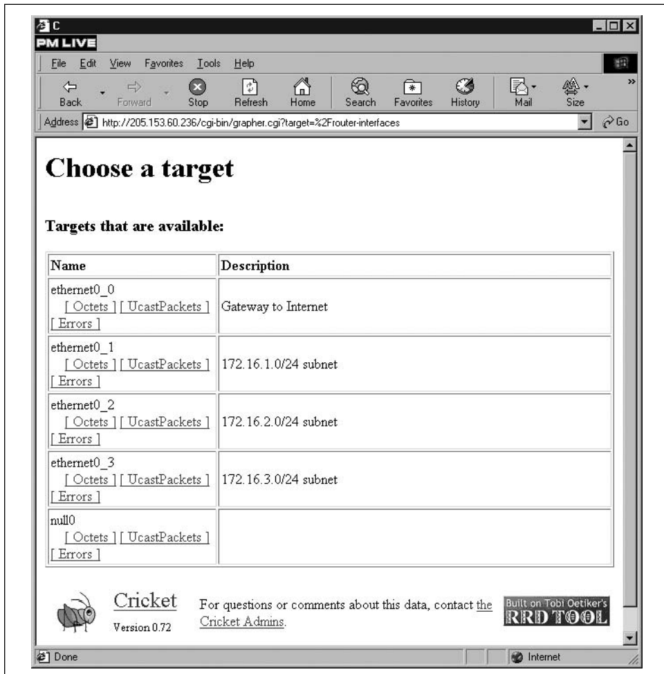
Figure 8-7. cricket router interfaces
