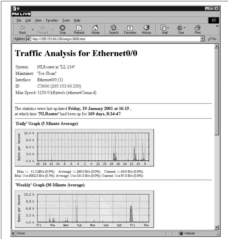
Figure 8-6. mrtg interface report
