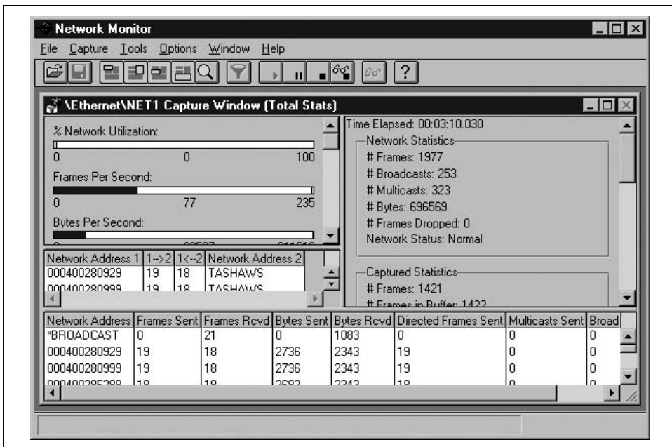
Figure 8-9. netmon traffic monitoring
