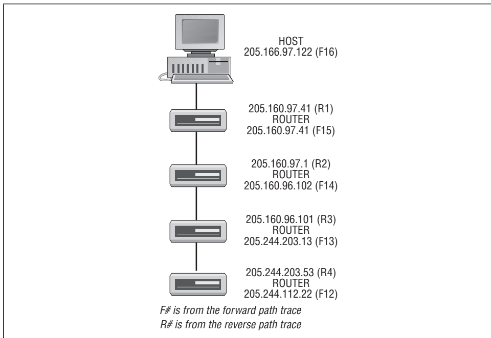
Figure 4-2. First four hops on reverse path
