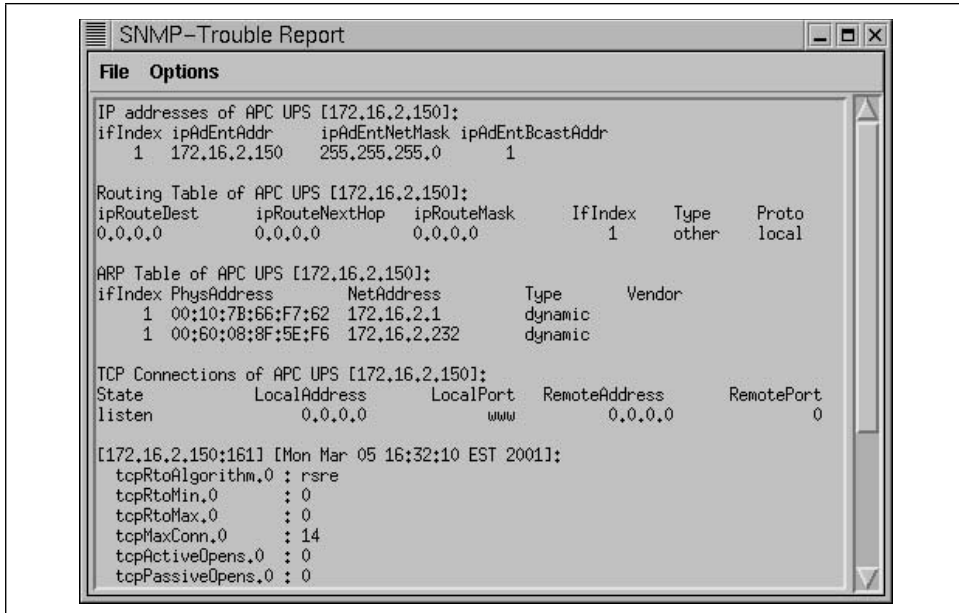
Figure 7-13. SNMP-Trouble reports
