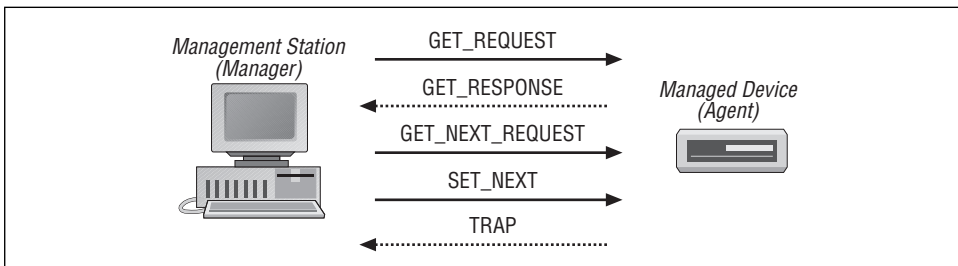
Figure 7-1. SNMP messages
