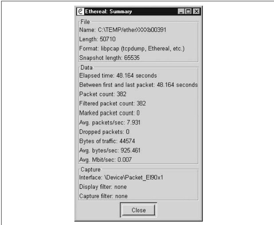
Figure 5-4. ethereal Summary
