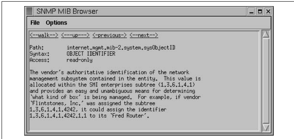
Figure 7-10. MIB Browser
