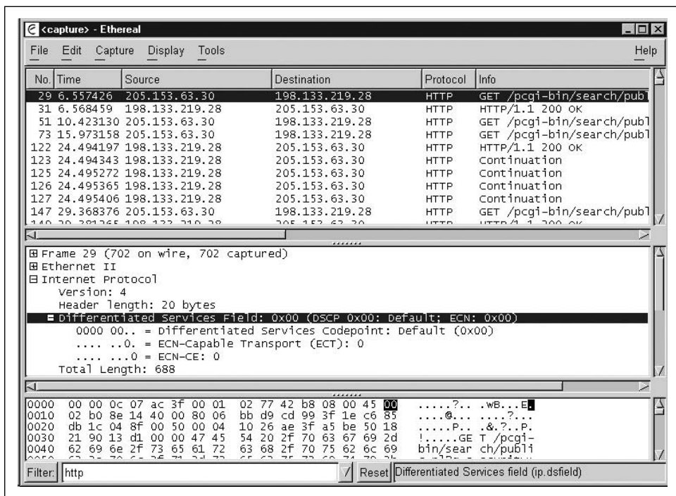
Figure 5-1. ethereal
