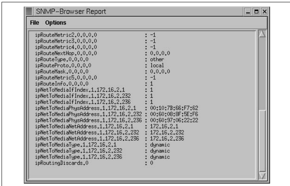
Figure 7-11. Walk for IP
