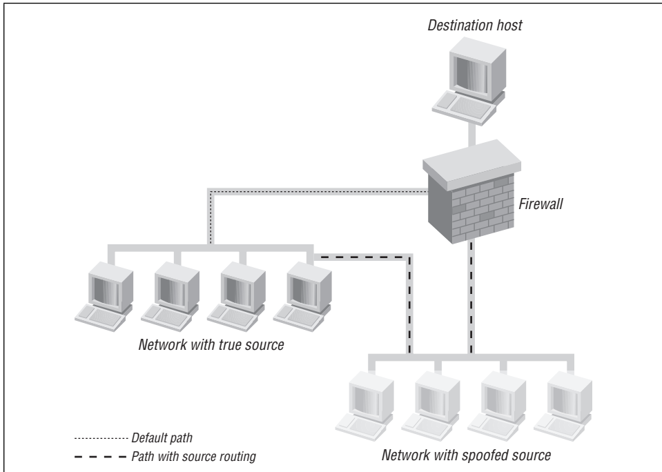
Figure 4-3. IP source spoofing
