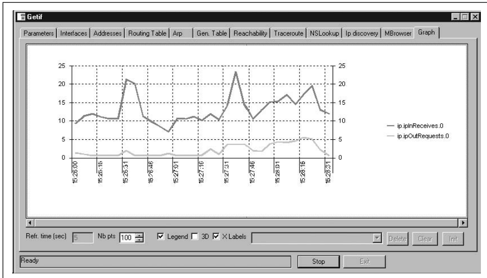
Figure 8-11. getif graph
