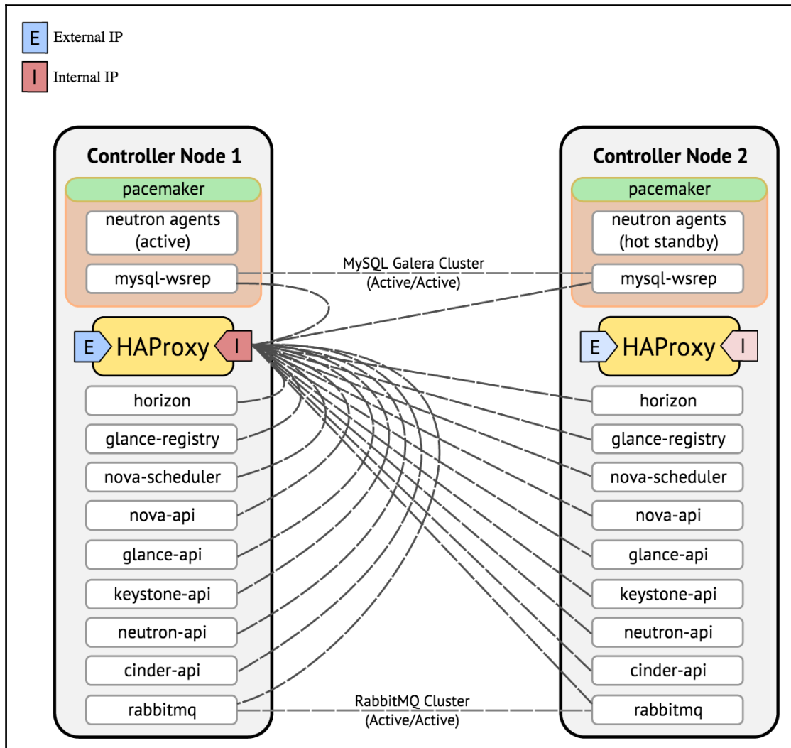
Mirantis OpenStack controller HA architecture – Mirantis
