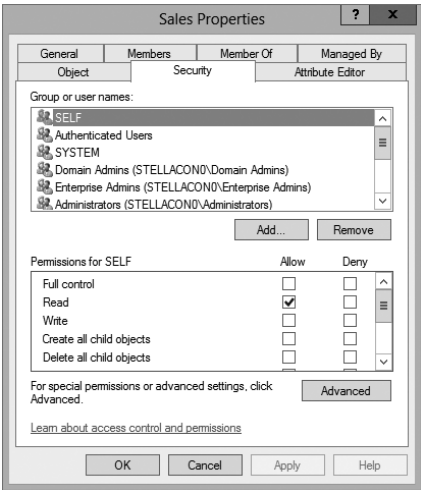
FIGURE 6.7 The ACL for an OU named Sales
