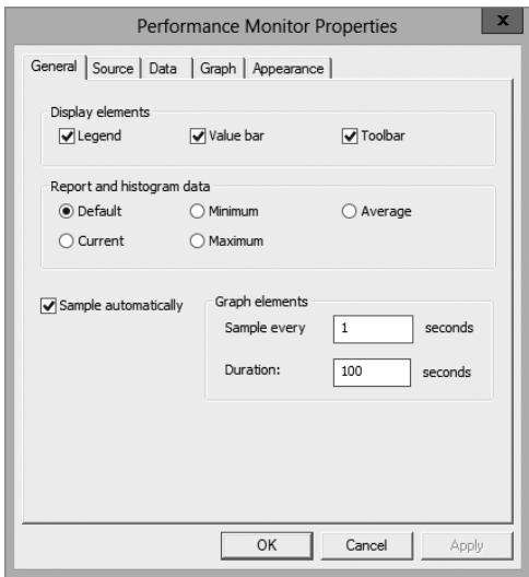
FIGURE 1.7 General tab of the Performance Monitor Properties dialog box
