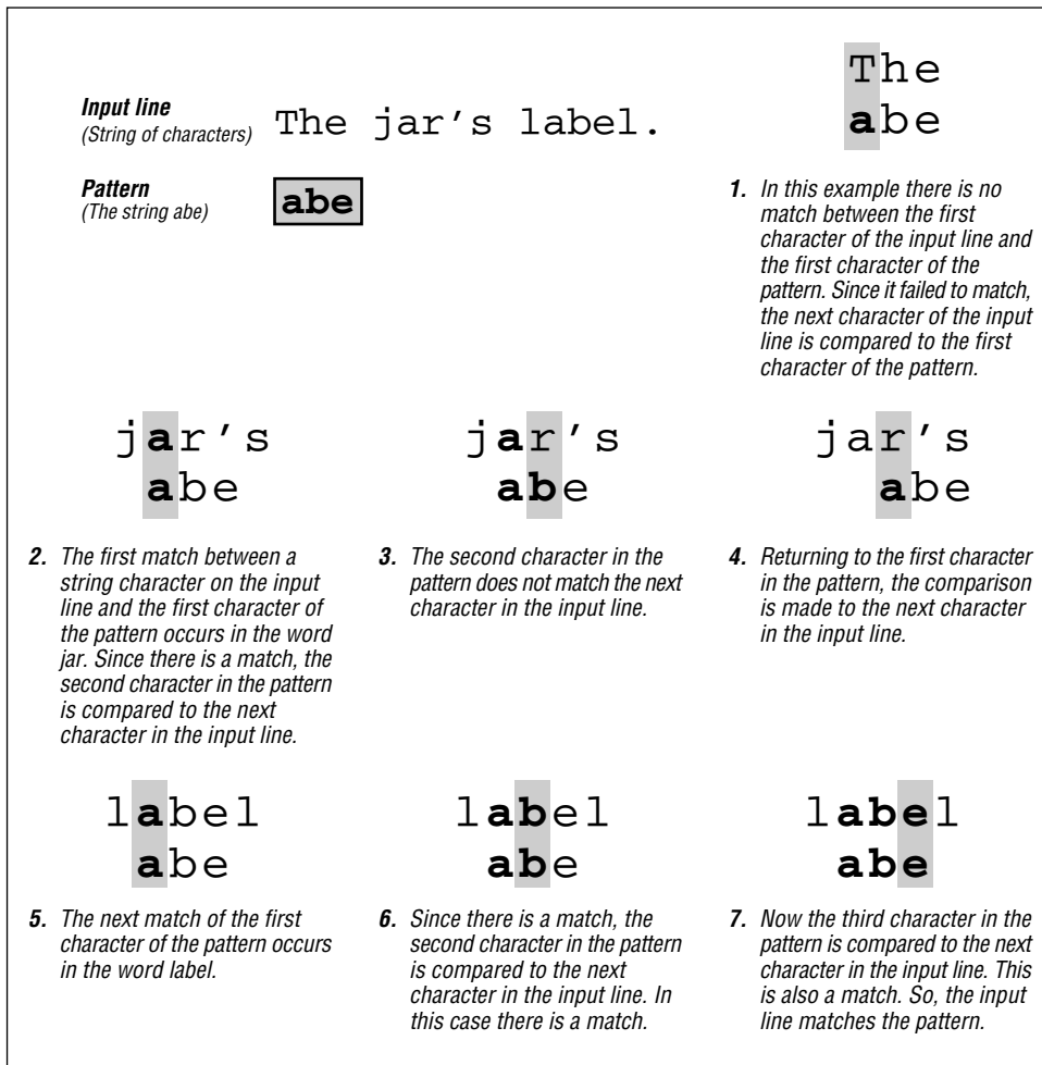
Figure 3-1: Interpreting a regular expression
