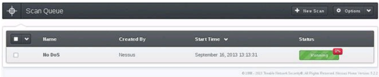
FIGURE 8.22 Scan Queue.
