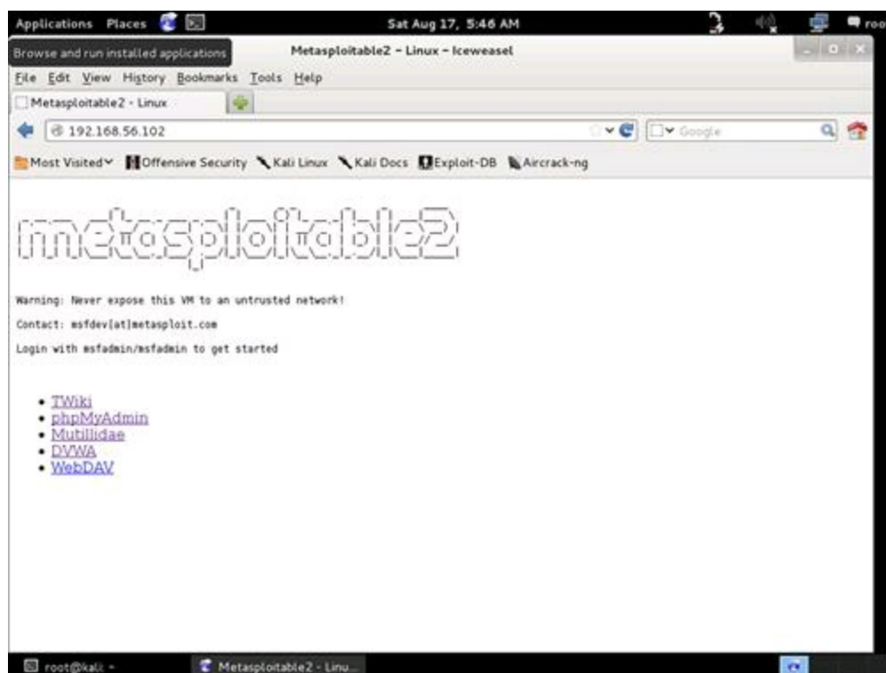
FIGURE 5.27 Web Interface.
