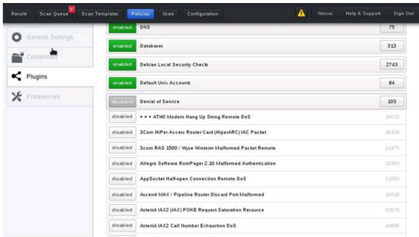
FIGURE 8.19 Removing DoS.
