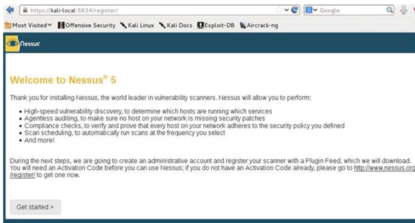
FIGURE 8.15 Nessus registration.
