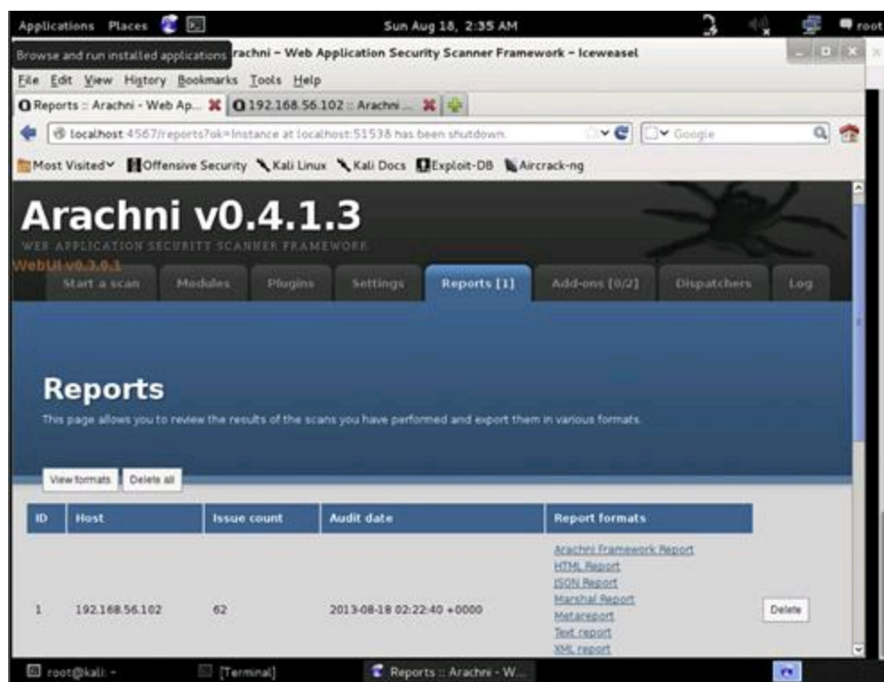
FIGURE 9.24 Arachni reporting.
