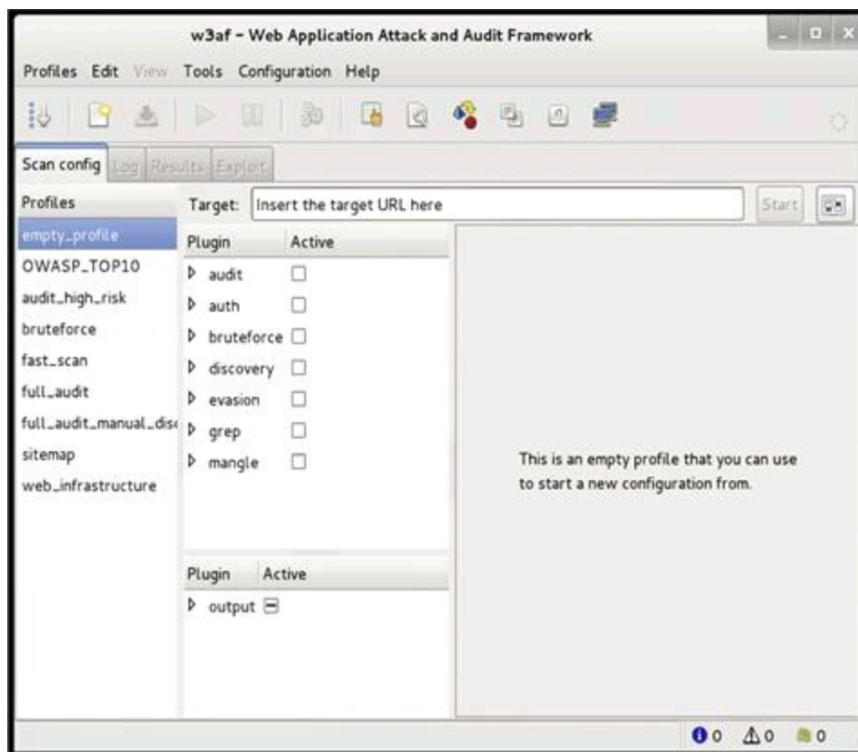
FIGURE 9.26 w3af console.
