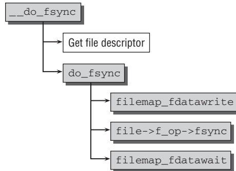
Figure 17-12: Code flow diagram for __do_sync .
