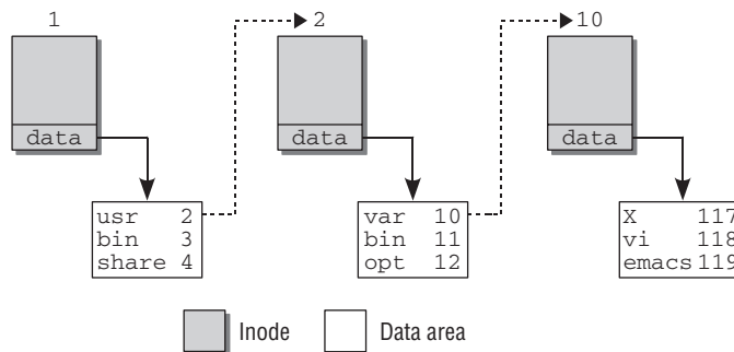
Figure 8-2: Lookup operation for /usr/bin/emacs .
