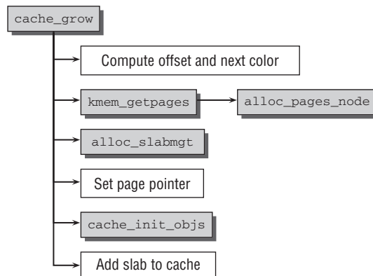
Figure 3-51: Code flow diagram for cache_grow .
