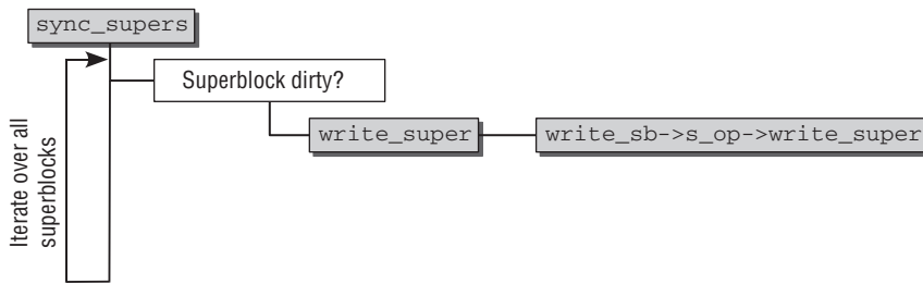
Figure 17-5: Code flow diagram for sync_supers .
