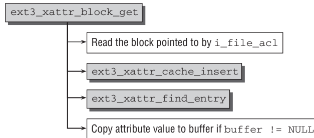
Figure 11-7: Code flow diagram for ext3_xattr_block_get .
