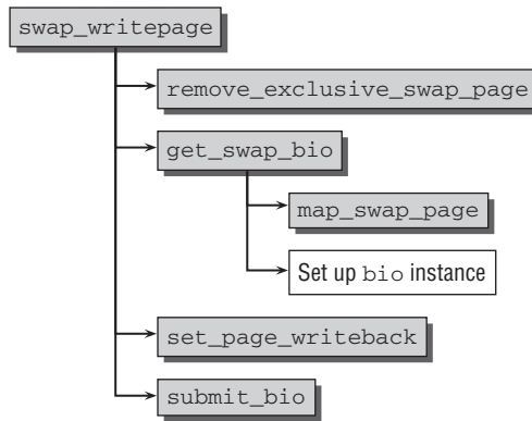
Figure 18-10: Code flow diagram for swap_writpage .
