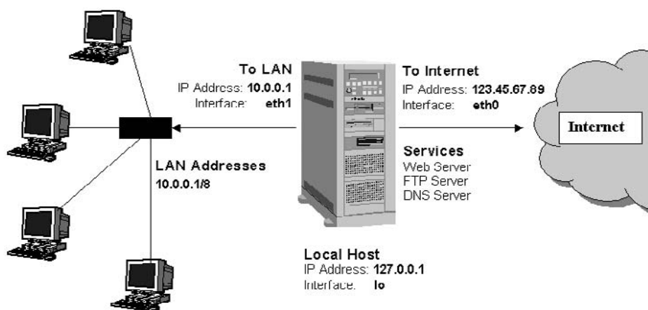
Figure 13-2: Using iptables as a firewall between the Internet and a LAN
