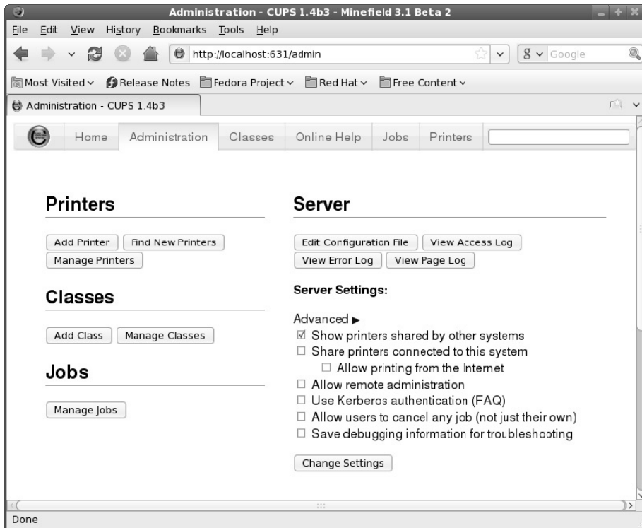
Figure 17-4: CUPS enables Web-based administration via port 631.
