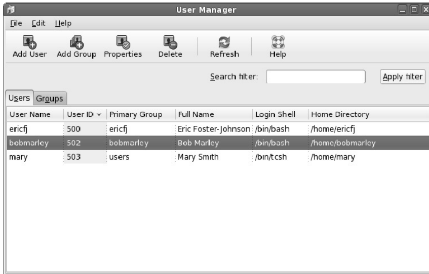
Figure 11-1: Manage users from the User Manager window.
