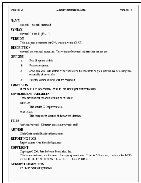
Figure 6-4: Man page formatting adds headers and lays out the page of text.
