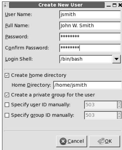
Figure 11-2: The Create New User window
