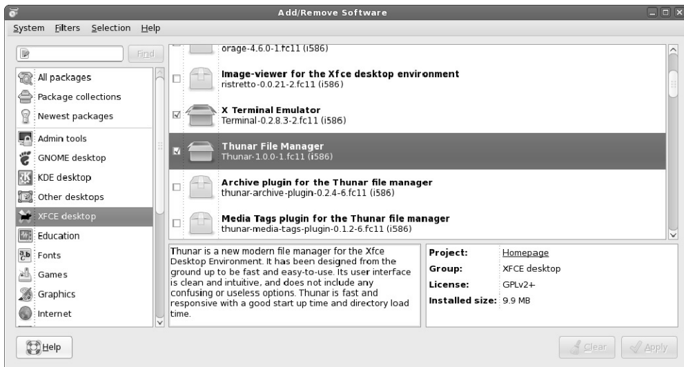
Figure 5-2: Get additional software packages using the PackageKit Add/Remove Software window.
