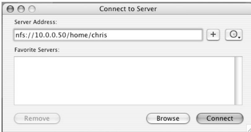
Figure 26-5: Connect to an NFS server from the Connect to Server window.
