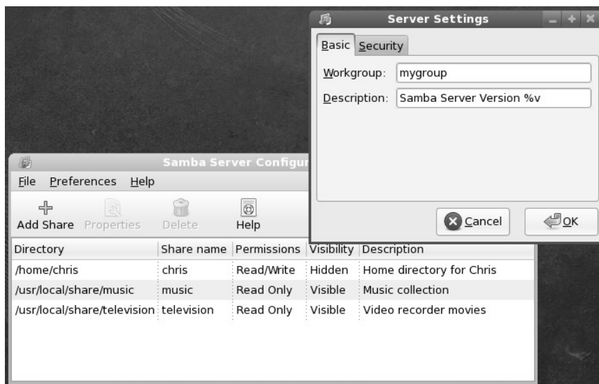
Figure 18-3: Define the workgroup and description for your Samba server.
