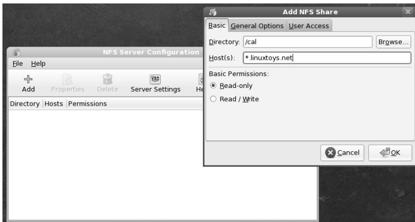
Figure 18-2: Identify a directory to share and access permissions with the NFS Server Configuration window.
