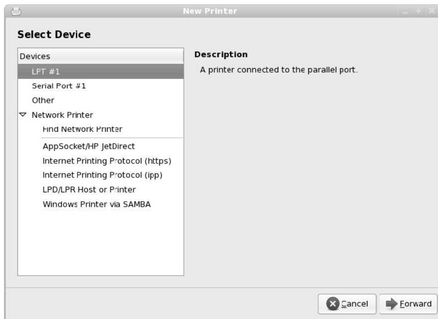
Figure 17-1: Add printers connected locally or remotely with the Printer Configuration window.
