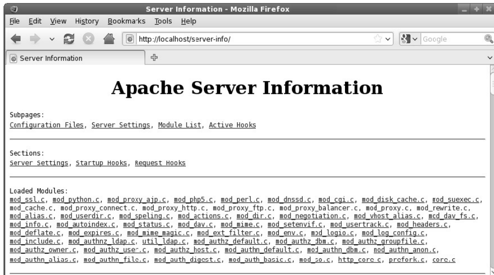
Figure 21-3: The server-info page displays server and module information.
