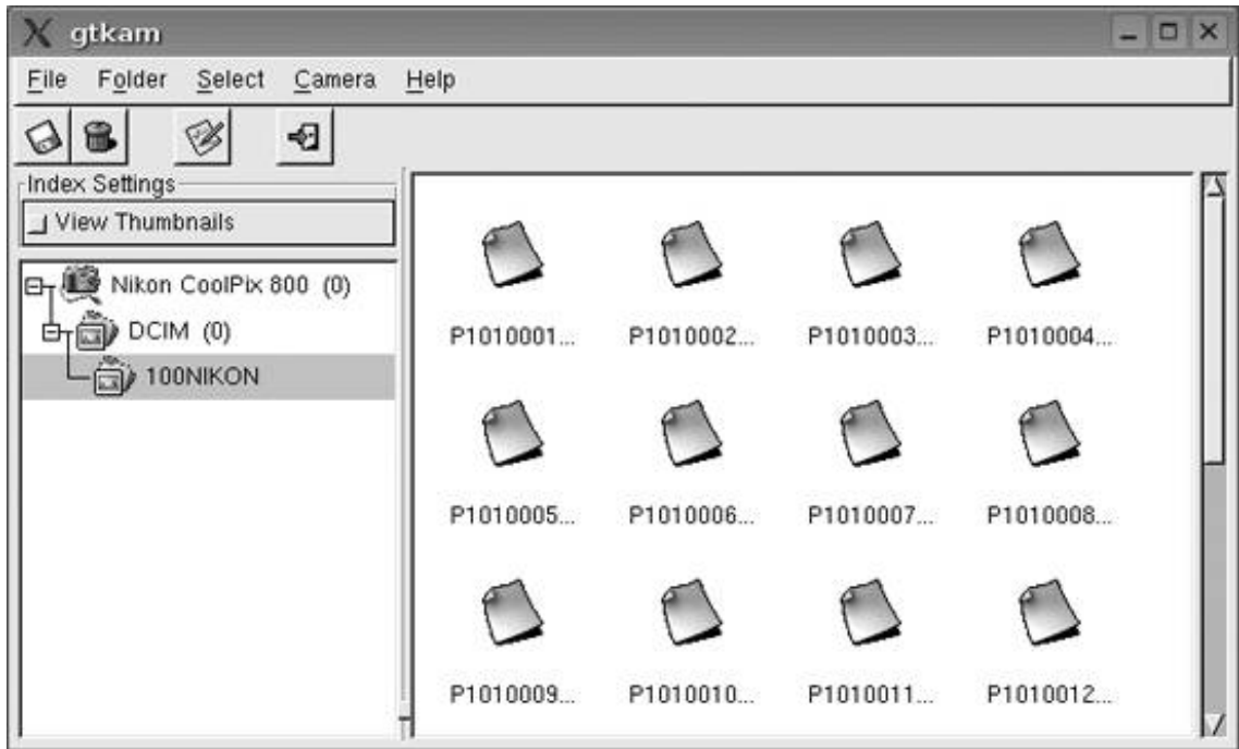
Figure 9-9. Gtkaam
