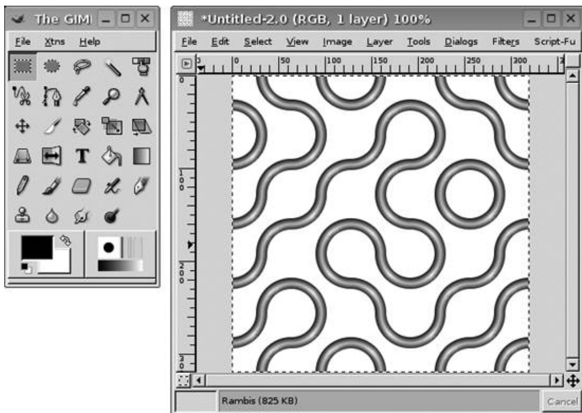
Figure 9-7. GIMP
