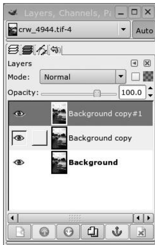
Figure 9-27. Layers dialog
