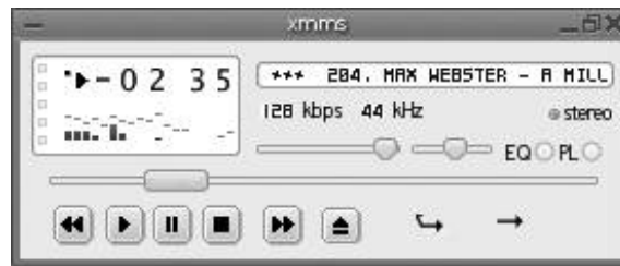
Figure 9-2. Xmms
