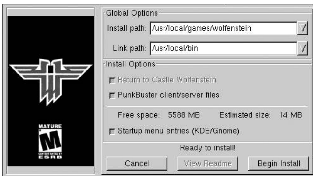
Figure 7-3. RTCW installer
