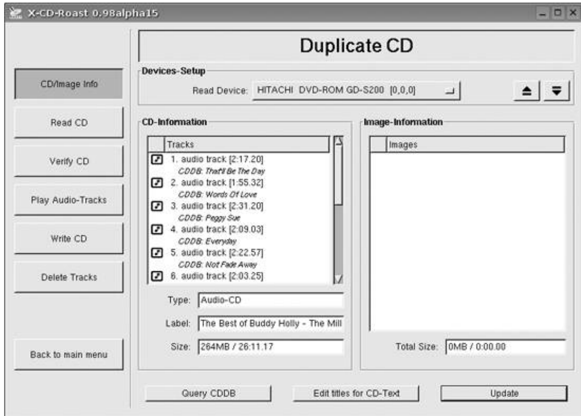
Figure 9-4. X-CD-Roast
