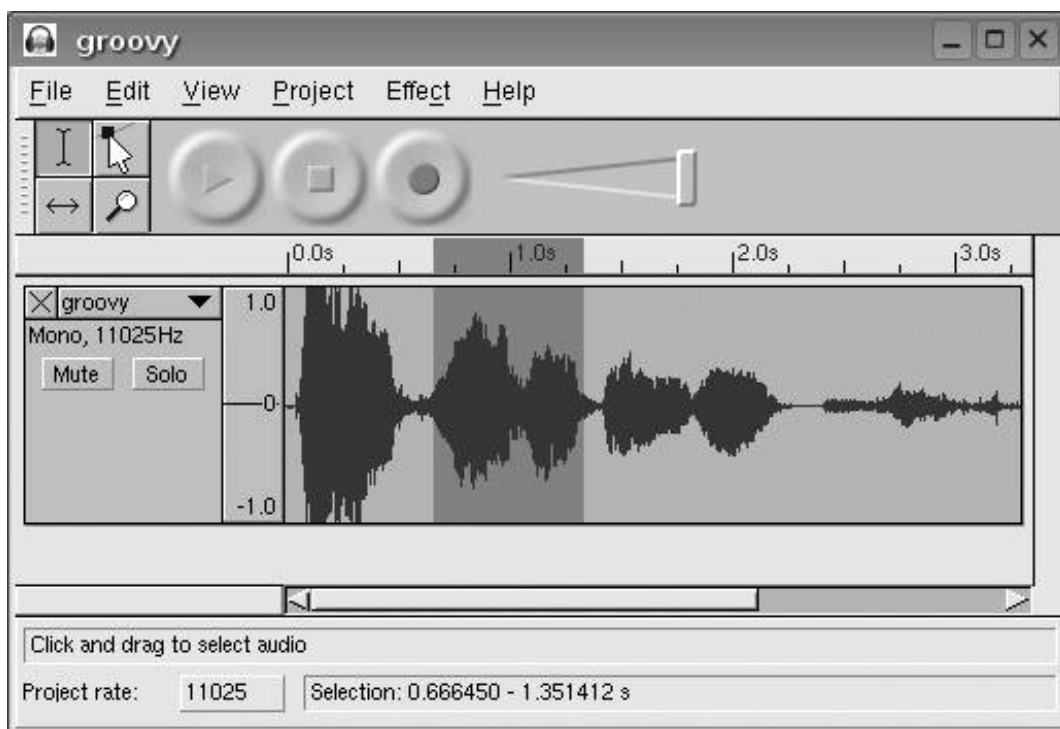
Figure 9-34. Audacity
