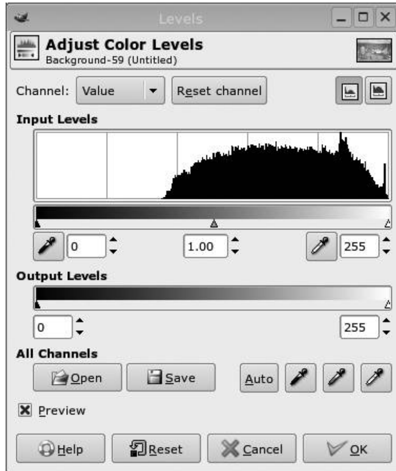
Figure 9-18. Levels dialog
