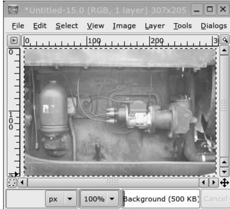
Figure 9-17. Original photo
