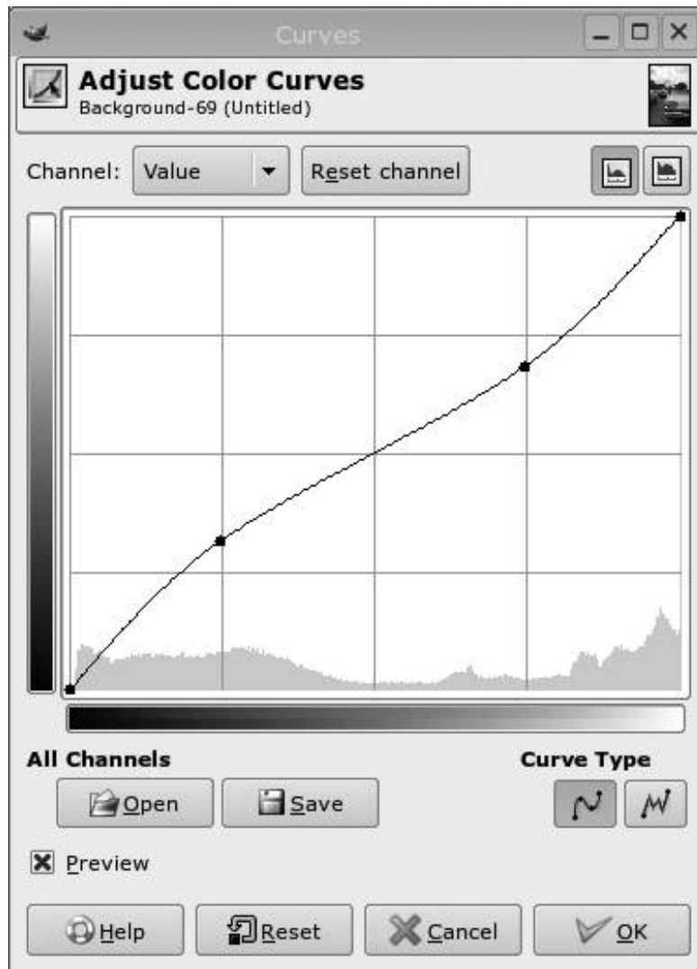
Figure 9-23. Contrast-decreasing curve
