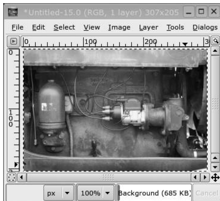
Figure 9-20. Level adjusted
