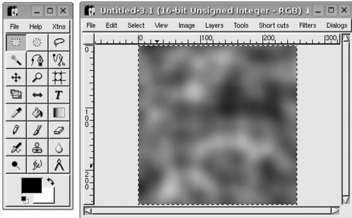
Figure 9-8. CinePaint
