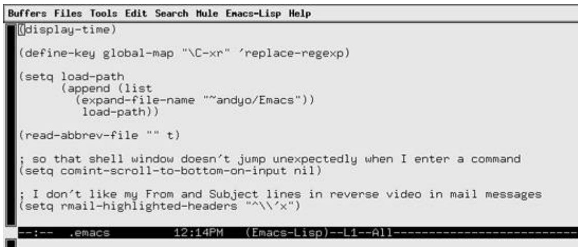
Figure 19-27. Emacs window
