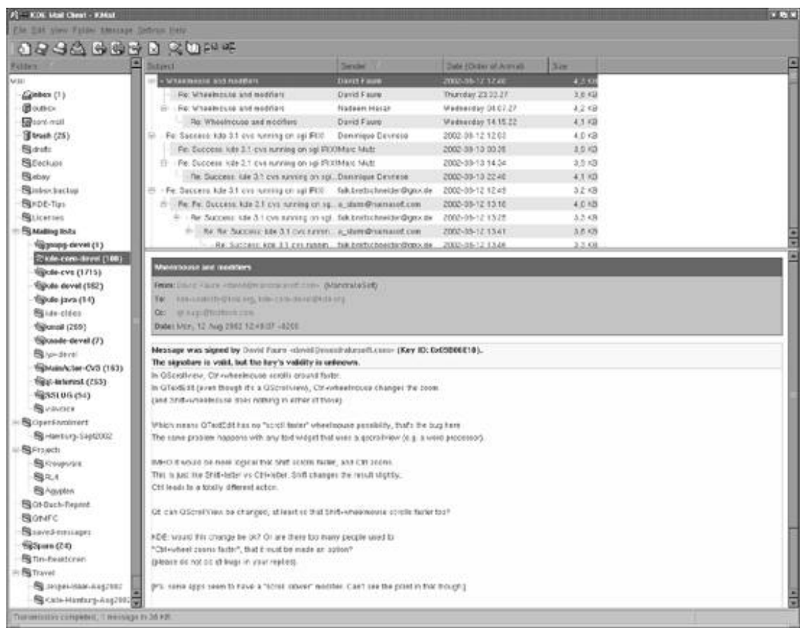
Figure 6-1. KMail mailer
