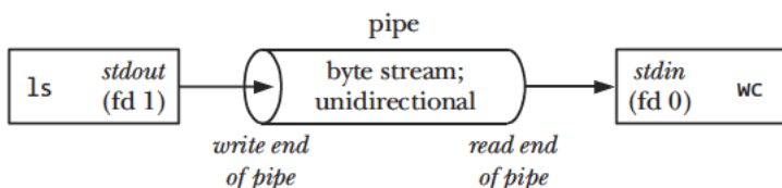
Figure 44-1: Using a pipe to connect two processes
