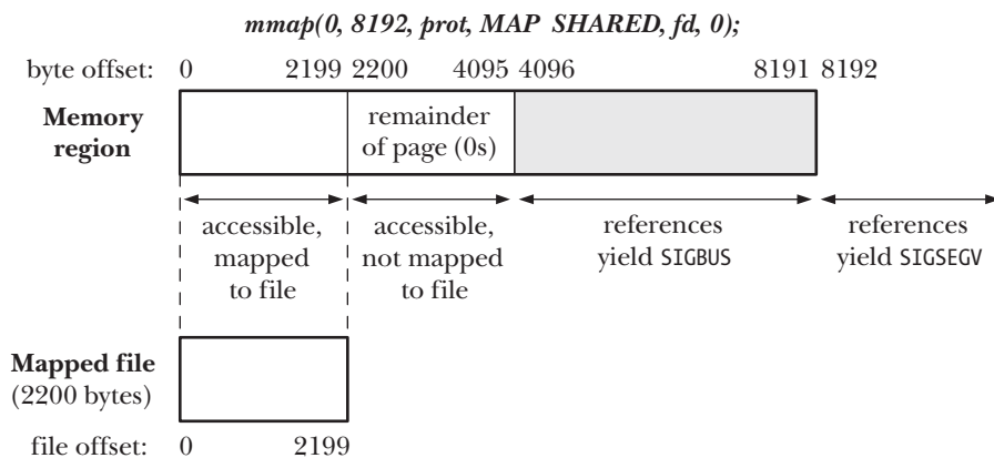
Figure 49-4: Memory mapping extending beyond end of mapped file
