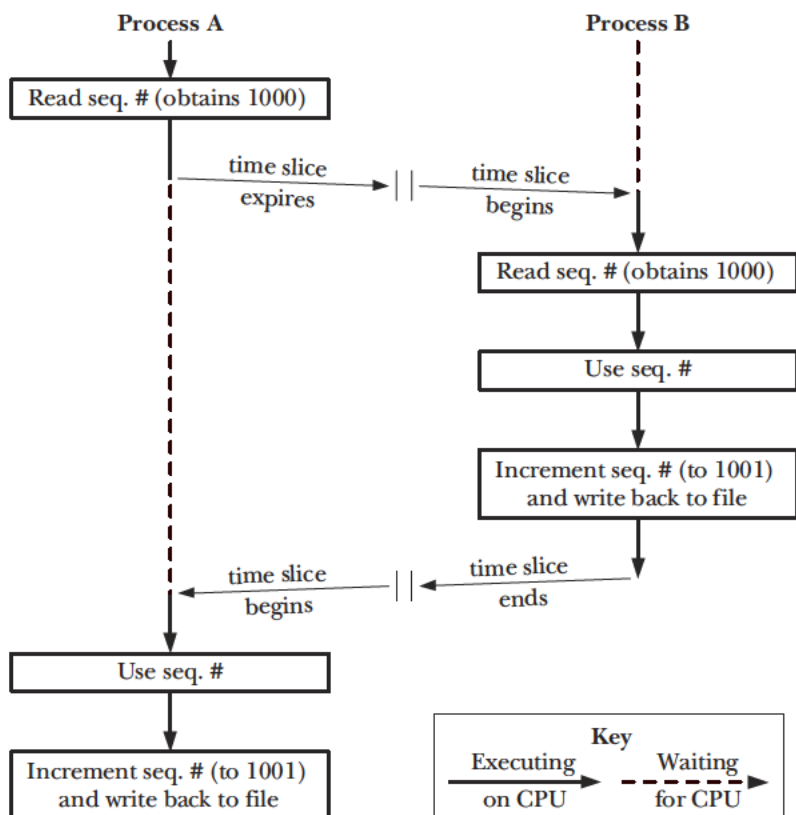
Figure 55-1: Two processes updating a file at the same time without synchronization
