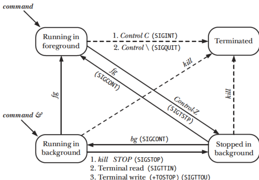
Figure 34-2: Job-control states
