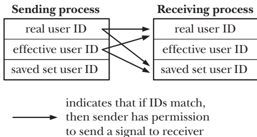
Figure 20-2: Permissions required for an unprivileged process to send a signal
