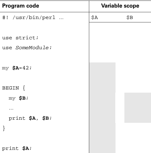
Figure 11.1 Illustration of variable scoping, without subroutines
