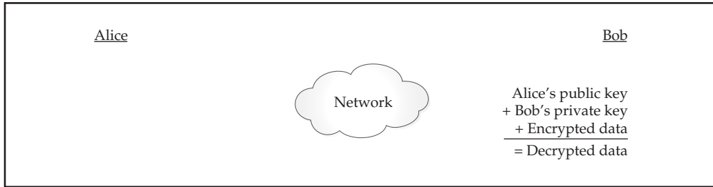
Figure 21-5. Bob uses Alice's public key, along with his private key, to verify and decrypt the data, respectively.
