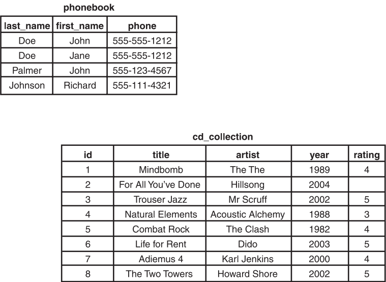
FIGURE 21.2 A single database can contain two tables—in this case, phonebook and cd_collection.
