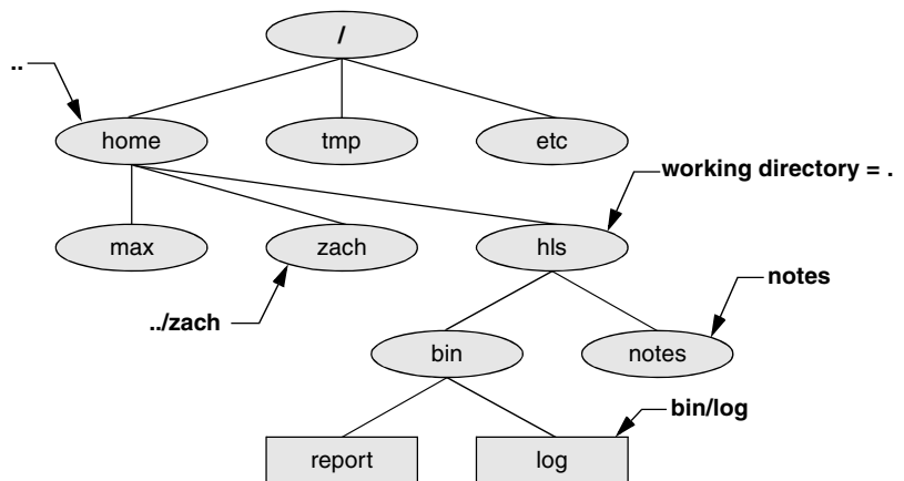
Figure 6-6 Relative pathnames
