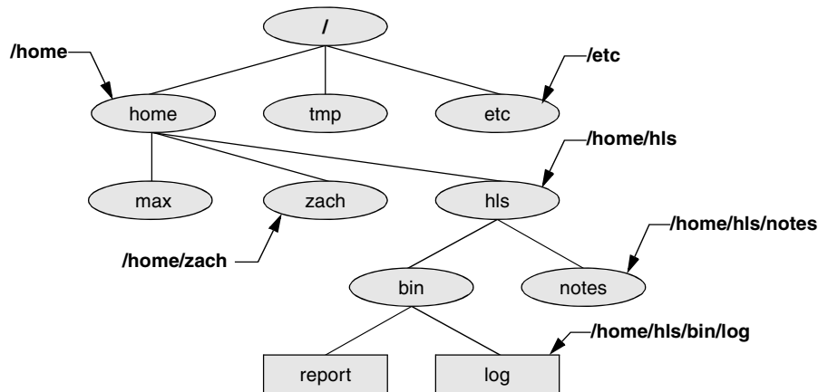
Figure 6-5 Absolute pathnames
