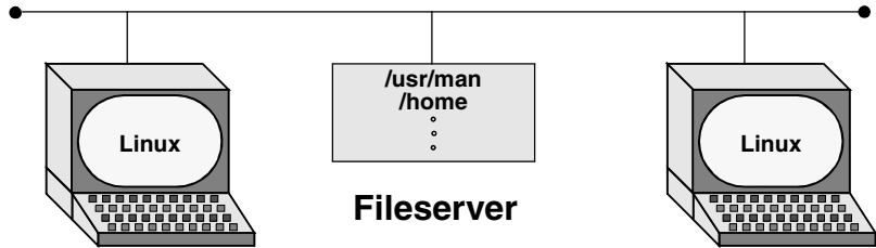
Figure 10-2 A fileserver
