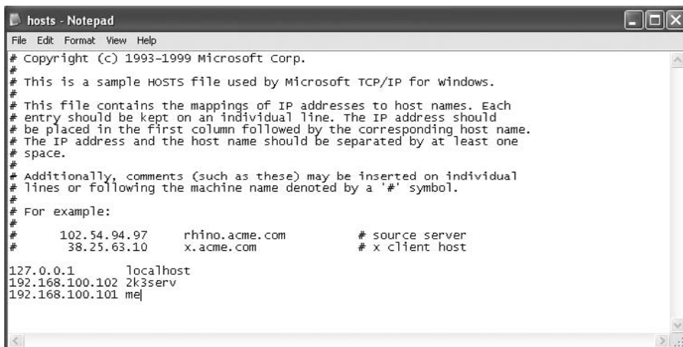
FIGURE 1-7 Modifying the hosts file with Notepad
