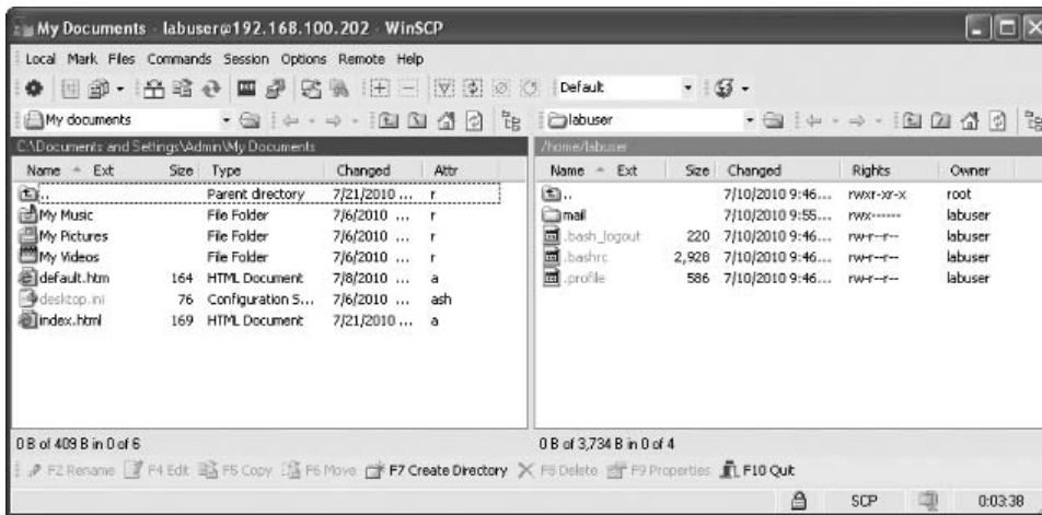
FIGURE 8-8 WinSCP interface
