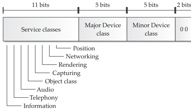
Figure 10-1 Bluetooth Class of Device/Service field
