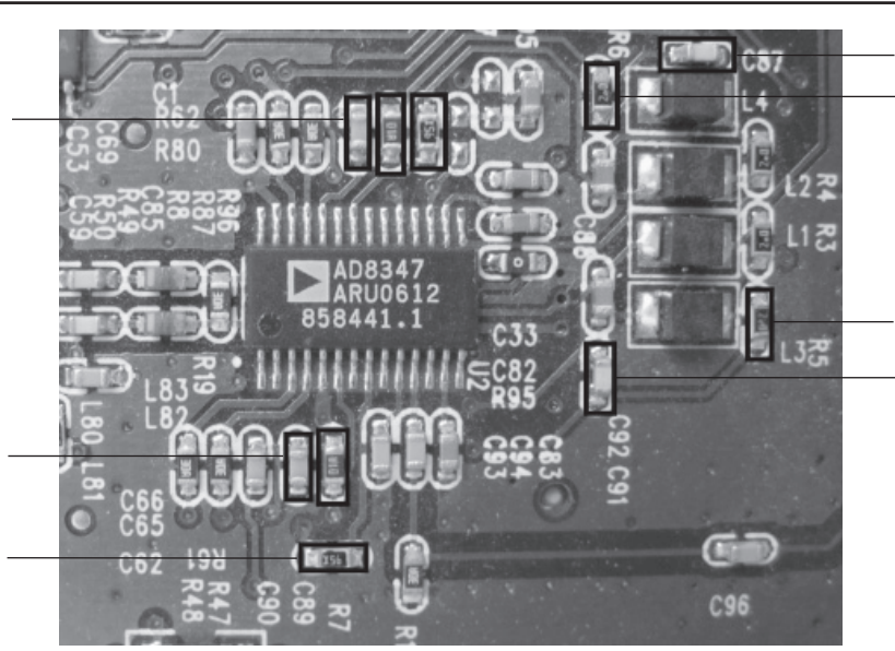
Figure 9-4 Locations for removing resistors and capacitors
