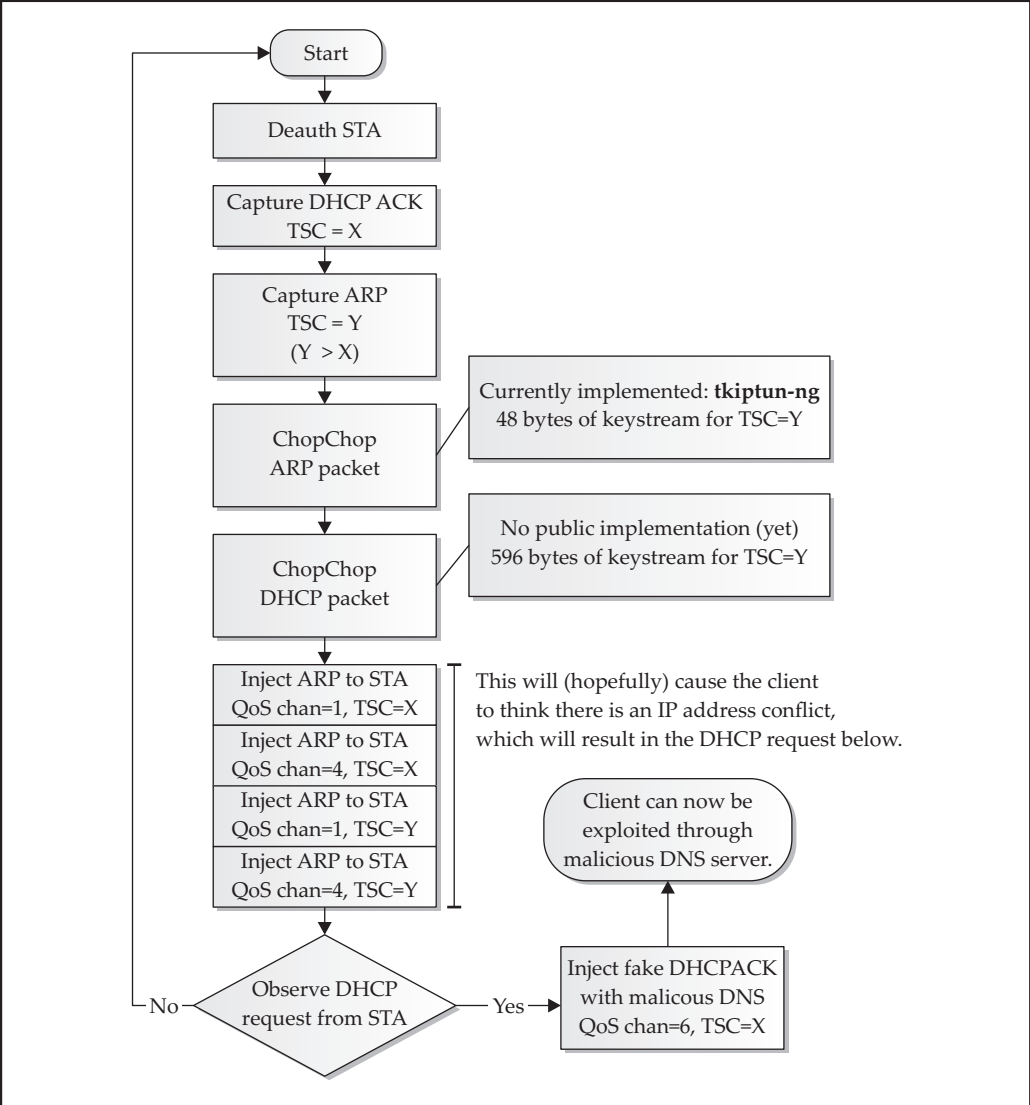
Figure 4-5 DHCP DNS attack
