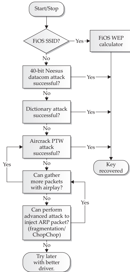
Figure 3-1 WEP cracking flowchart
