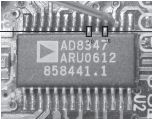
Figure 9-6 Leg lifter inserted underneath pin 18
