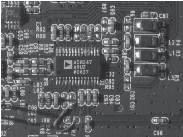
Figure 9-7 Completed RFX2400 modification
