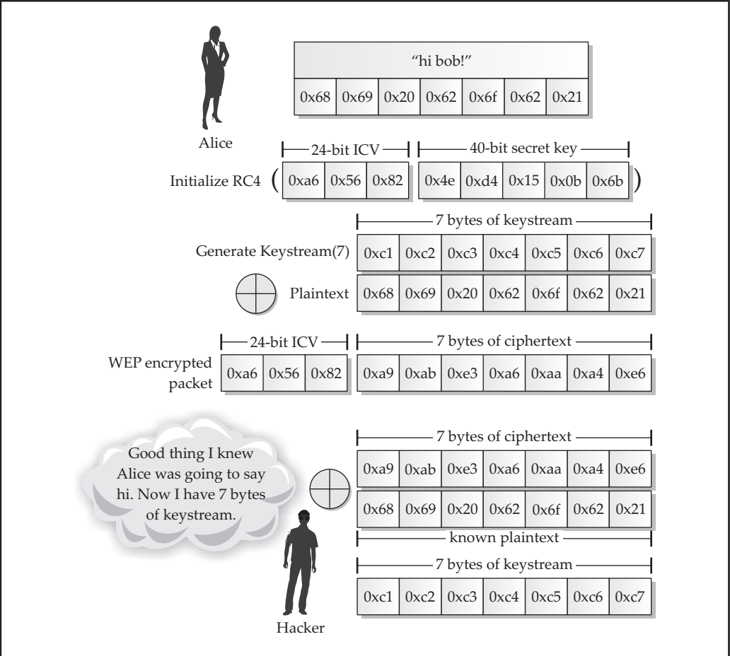
Figure 3-3 WEP encryption example
