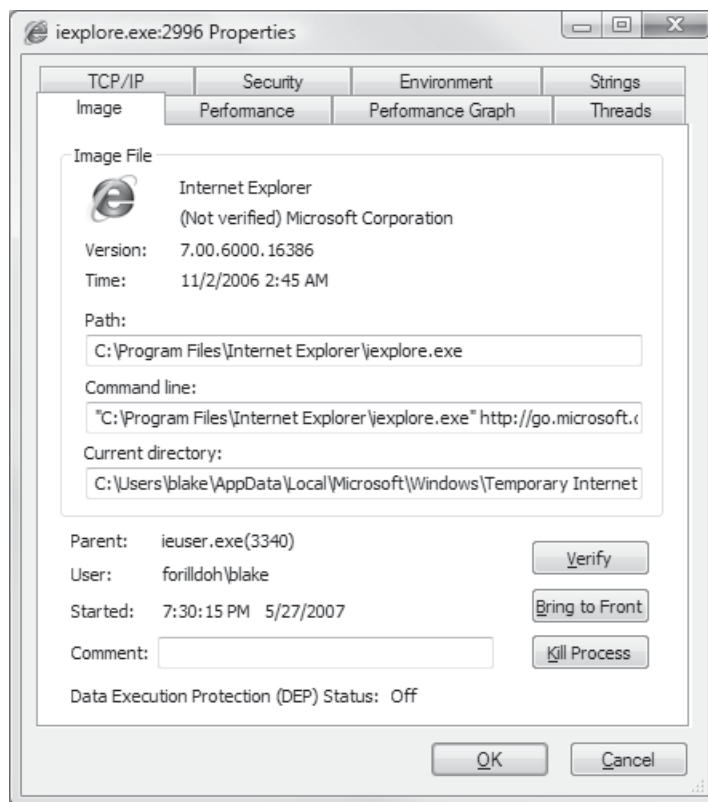
Figure 6-11 Internet Explorer with DEP disabled by default
