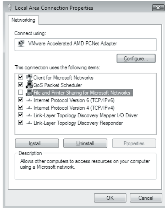
Figure 4-5 Disabling SMB completely on Vista, over both TCP 139 and 445
