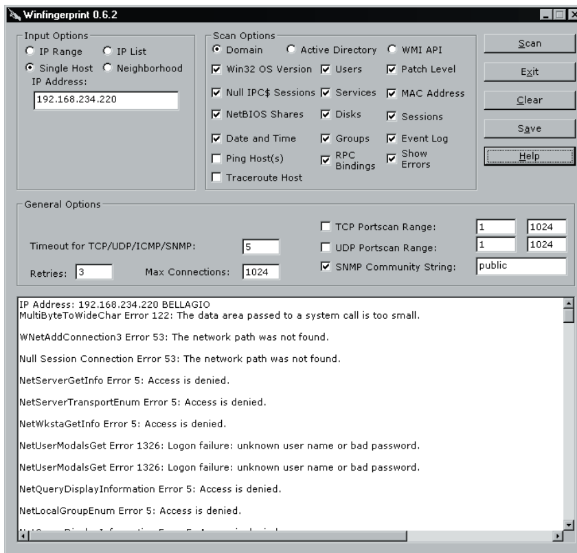
Figure 4-10 Winfingerprint enumerates a Windows Server 2008 Enterprise domain controller.
