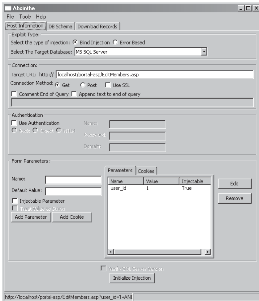
Figure 9-8 Absinthe can automate SQL injection and error-based data theft attacks.
