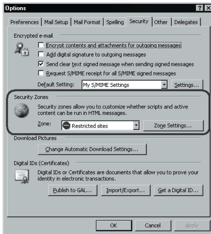
Figure 10-7 Configuring Outlook to use the Restricted Sites zone when browsing
