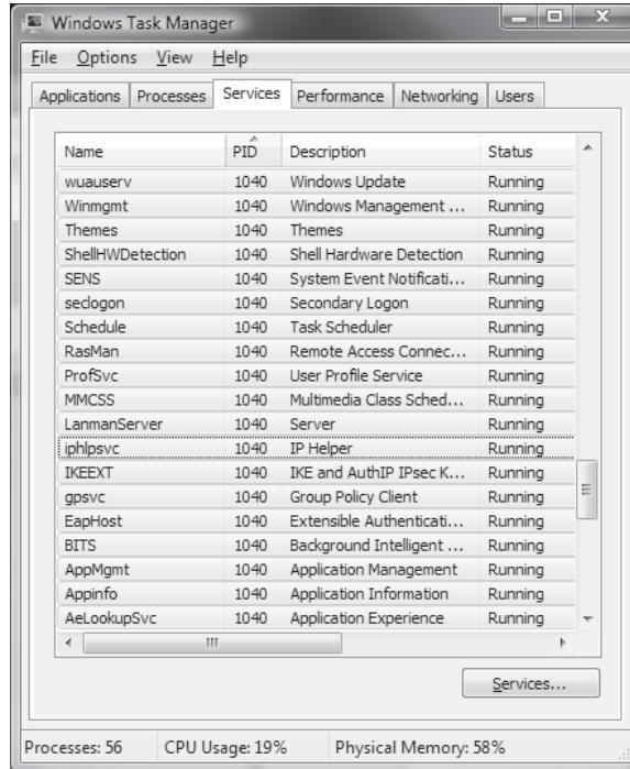
Figure 12-5 Nineteen services sharing a single PID
