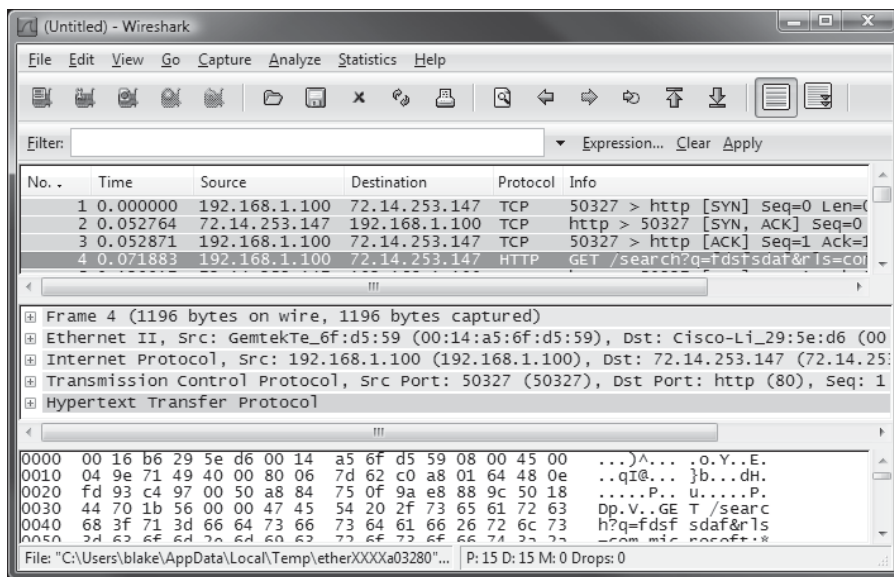
Figure 6-2 Select an HTTP GET request.
