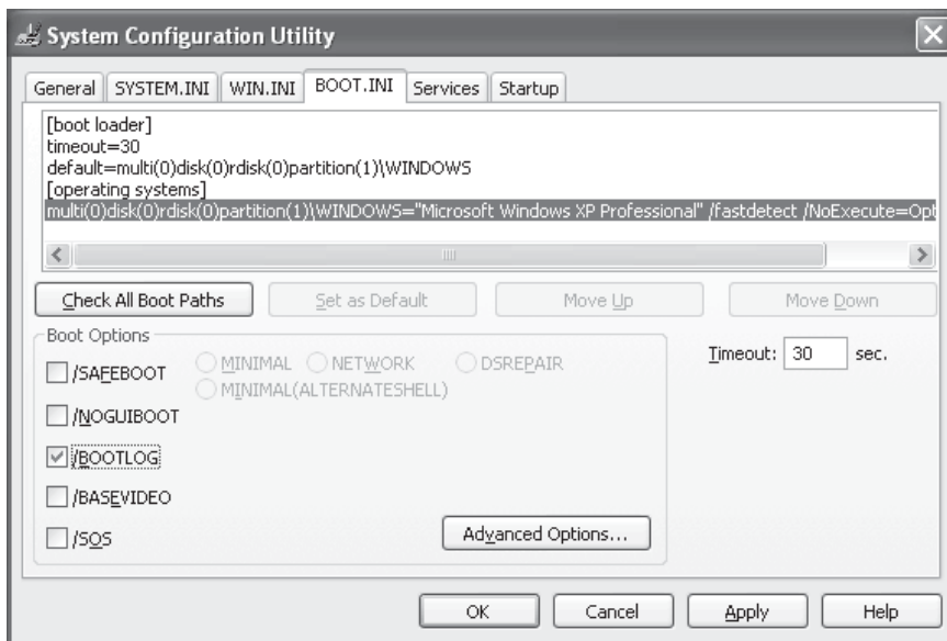
Figure 8-12 Using msconfig.exe to enable boot logging on Windows XP
