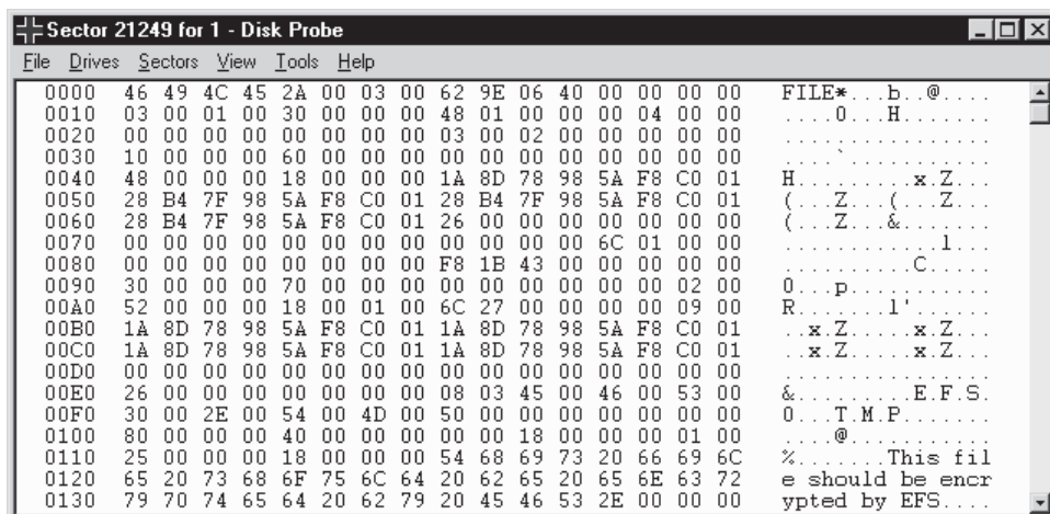
Figure 11-4 efs0.tmp open in dskprobe, revealing the cleartext content of the file
