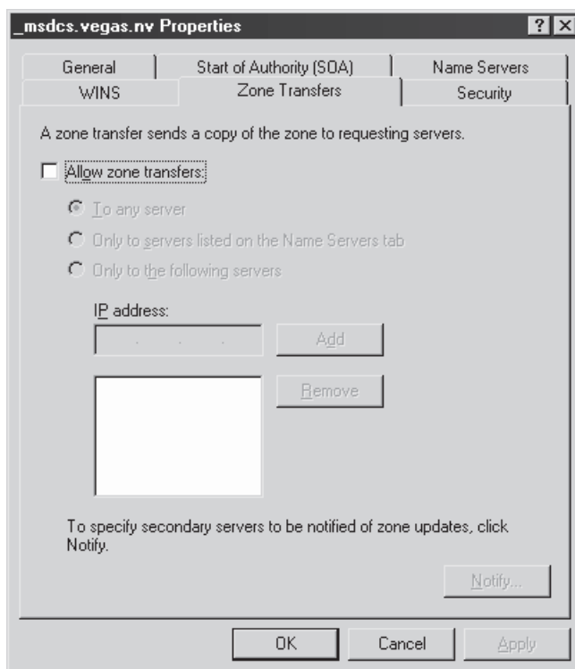
Figure 4-6 Windows Server 2003 default DNS settings disable zone transfers—hurrah for default security!
