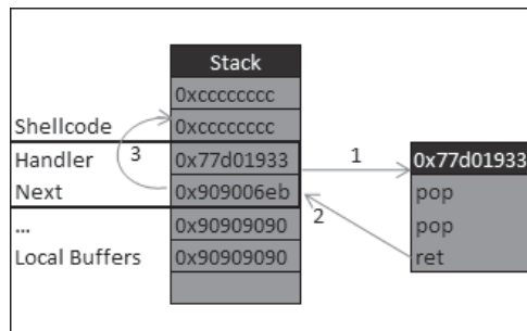
Figure 12-12 Exploiting SEH overwrites
