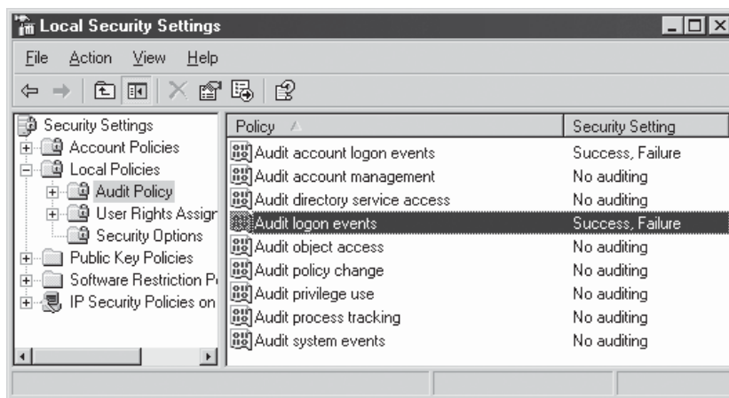
Figure 5-4 Enabling auditing of logon failure events can provide indication of password-guessing attacks.
