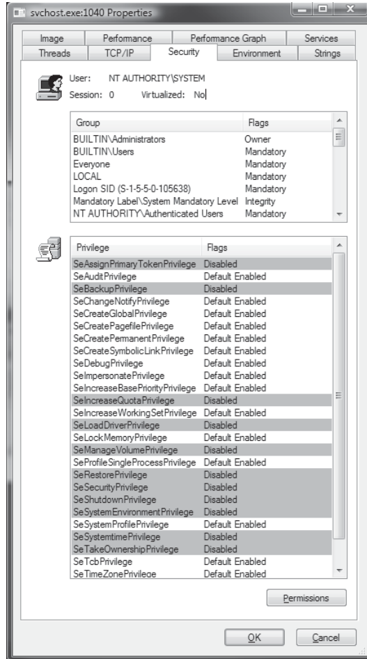
Figure 12-6 Aggregate of all privileges in service group
