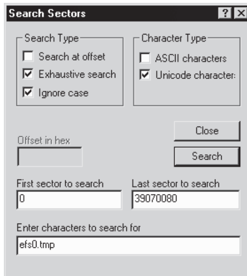
Figure 11-3 Dskprobe searches the physical disk for the string efs0.tmp.
