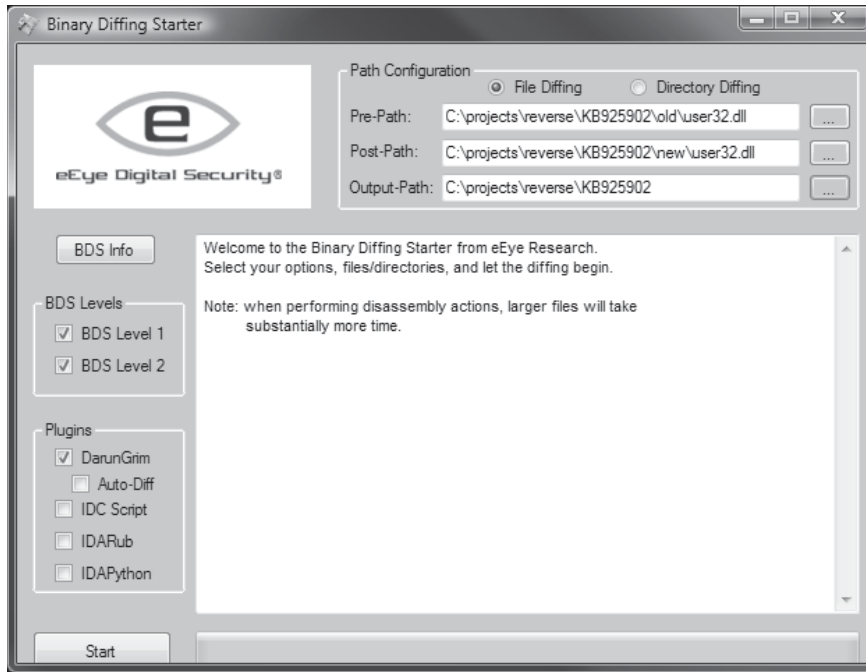
Figure 6-4 Binary Diffing Starter setup
