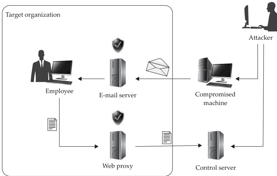
Figure 16-2 Content-type attack process
