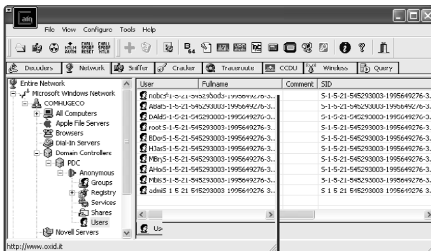
Figure 6-4 PDC User Enumeration with Cain
