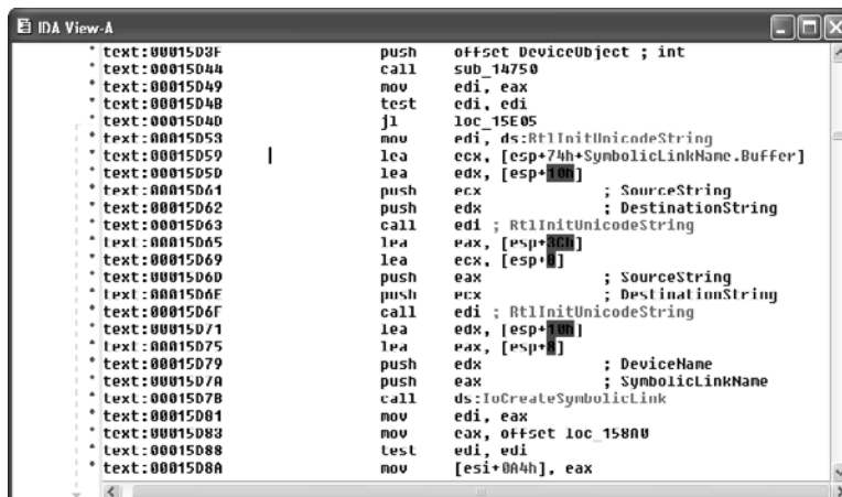
Figure 20-3 IDA Pro naming and commenting
