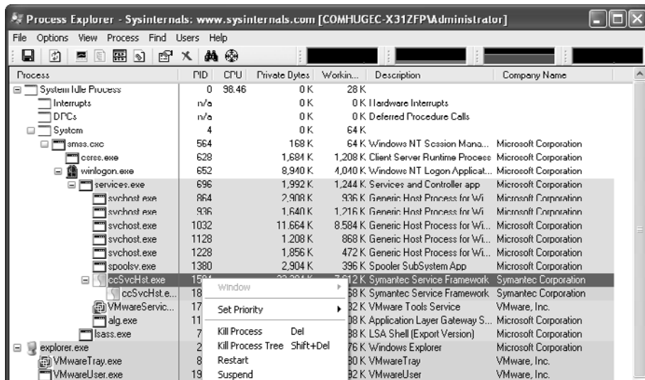
Figure 6-3 Process Explorer
