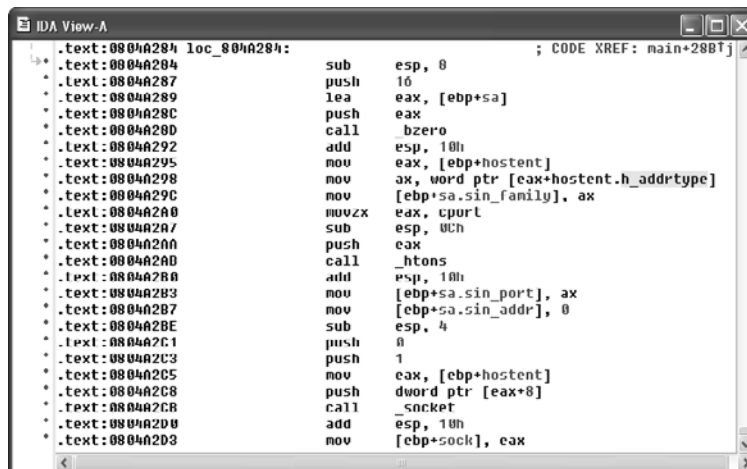
Figure 20-7 Applying IDA Pro structure templates
