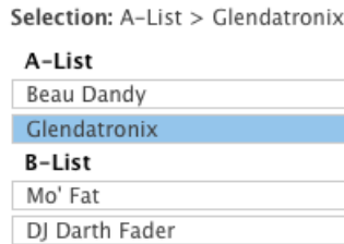
Figure 8.4. Delegating events
