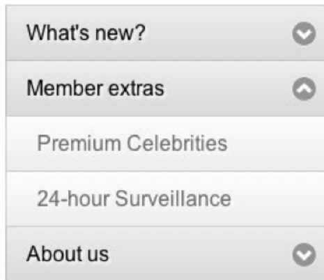
Figure 5.2. Open/closed indicators
