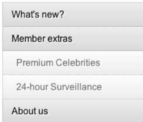
Figure 5.1. Expandable menus
