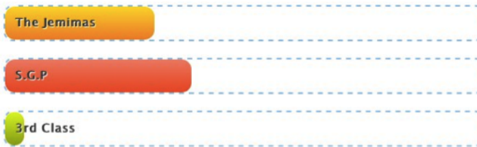
Figure 9.1. Animation starting
