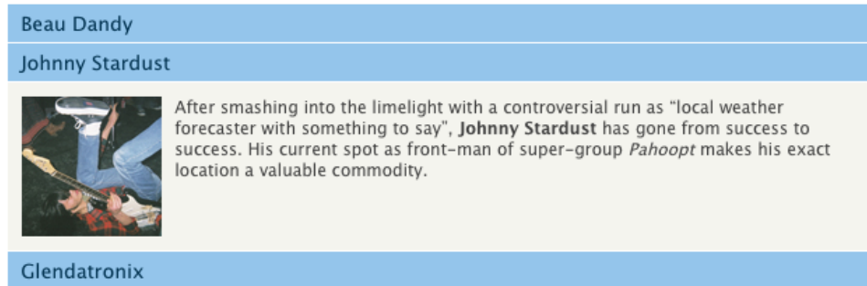
Figure 3.3. Biography panes
