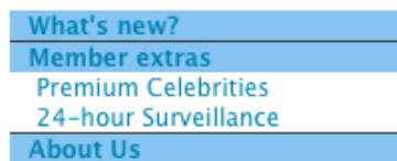
Figure 5.1. Expandable menus
