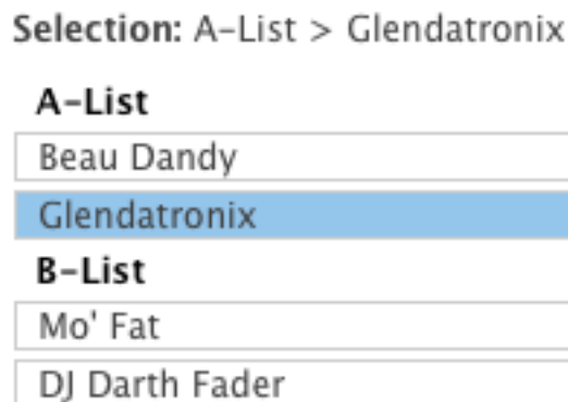
Figure 8.4. Delegating events
