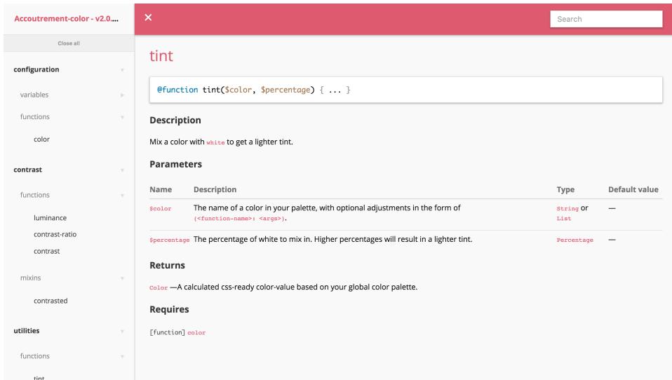
Figure 10.1. SassDoc Output
