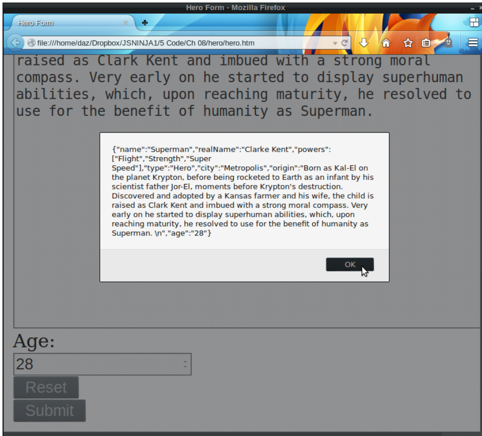
Figure 8.6. Hero JSON
