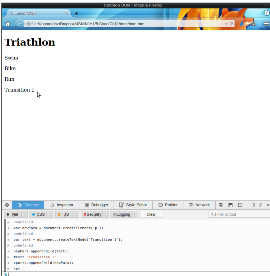
Figure 6.5. Append child
