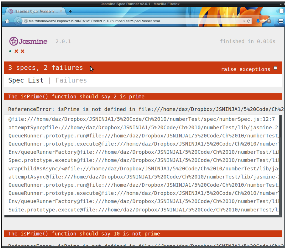
Figure 10.5. Failing again
