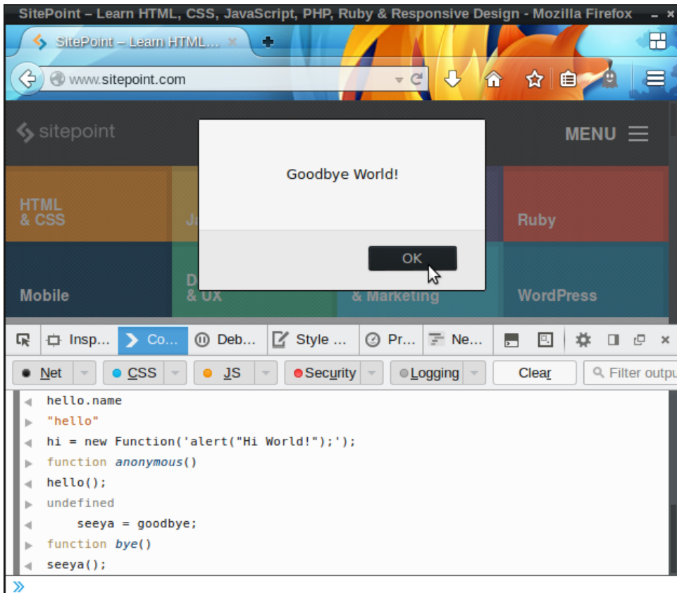
Figure 4.2. Goodbye World!
