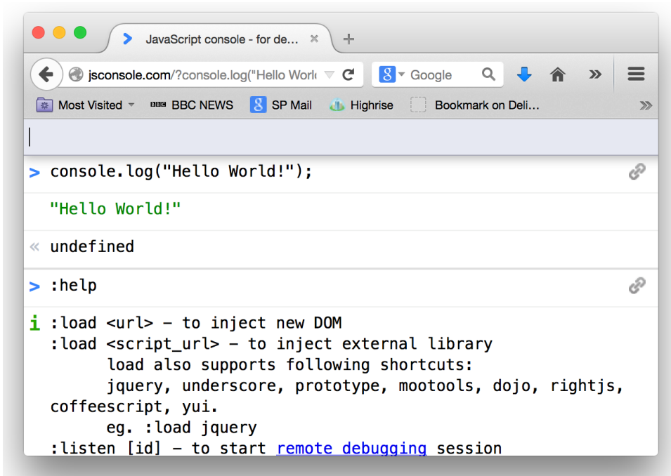
Figure 1.1. "Hello, world!"
