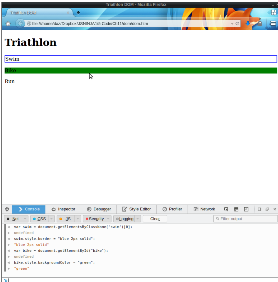
Figure 6.11. Green background
