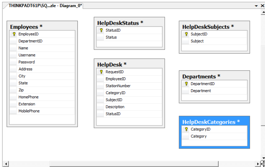
Figure 7.19. Visualizing data tables using a diagram
