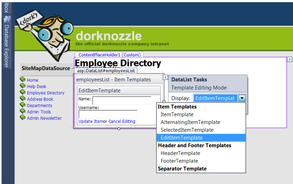
Figure 10.9. Building the DataList 's templates visually
