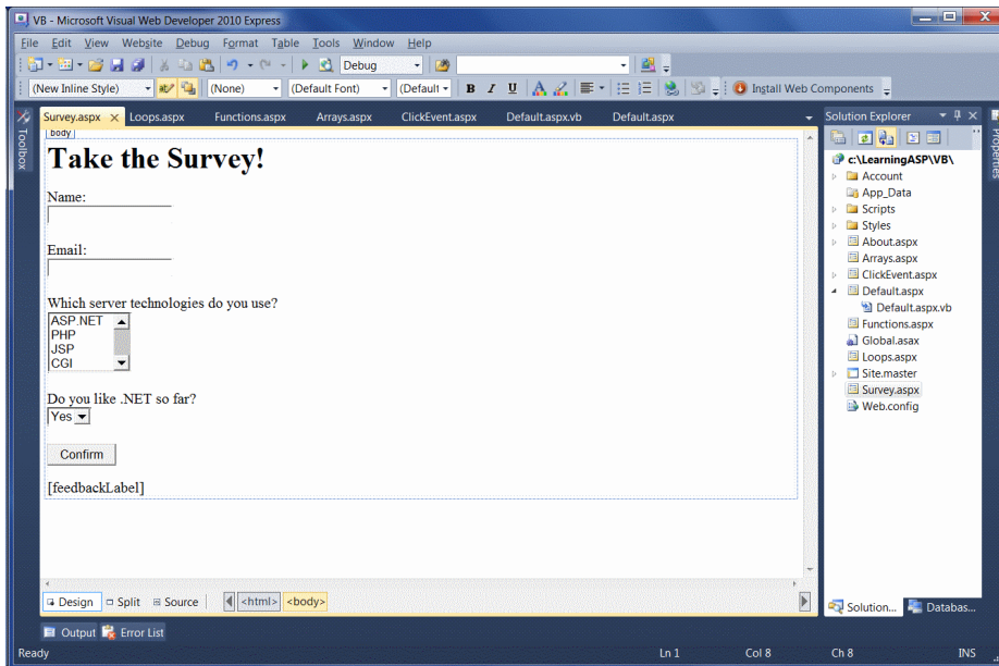
Figure 4.1. A simple form that uses HTML server controls
