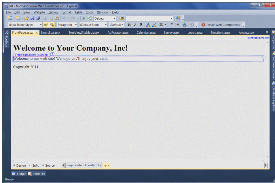
Figure 4.15. Design mode shows the editable areas of a form that uses a master page
