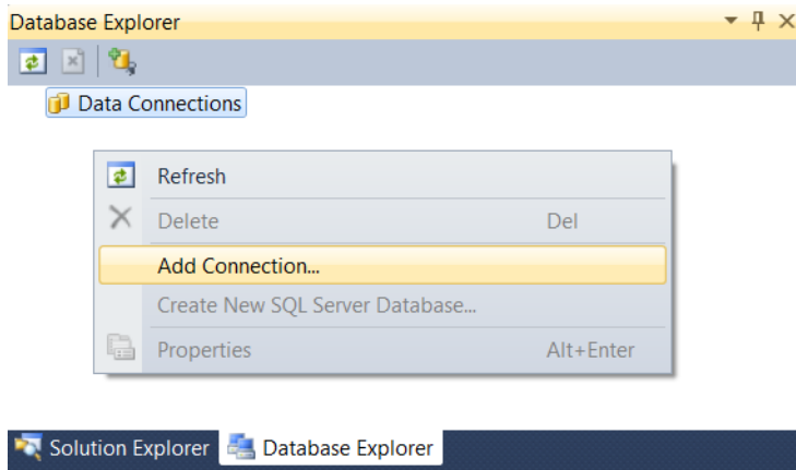
Figure 7.2. Adding a new database connection
