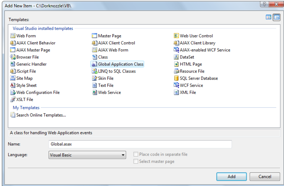
Figure 5.17. Creating Global.asax
