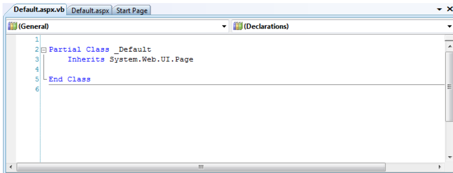
Figure 5.6. Editing Default.aspx.vb
