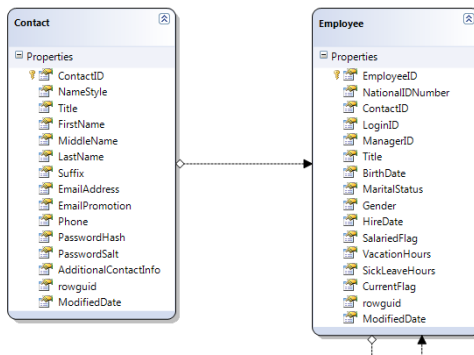
Figure 15.4. Dropping the contacts table onto DBML designer
