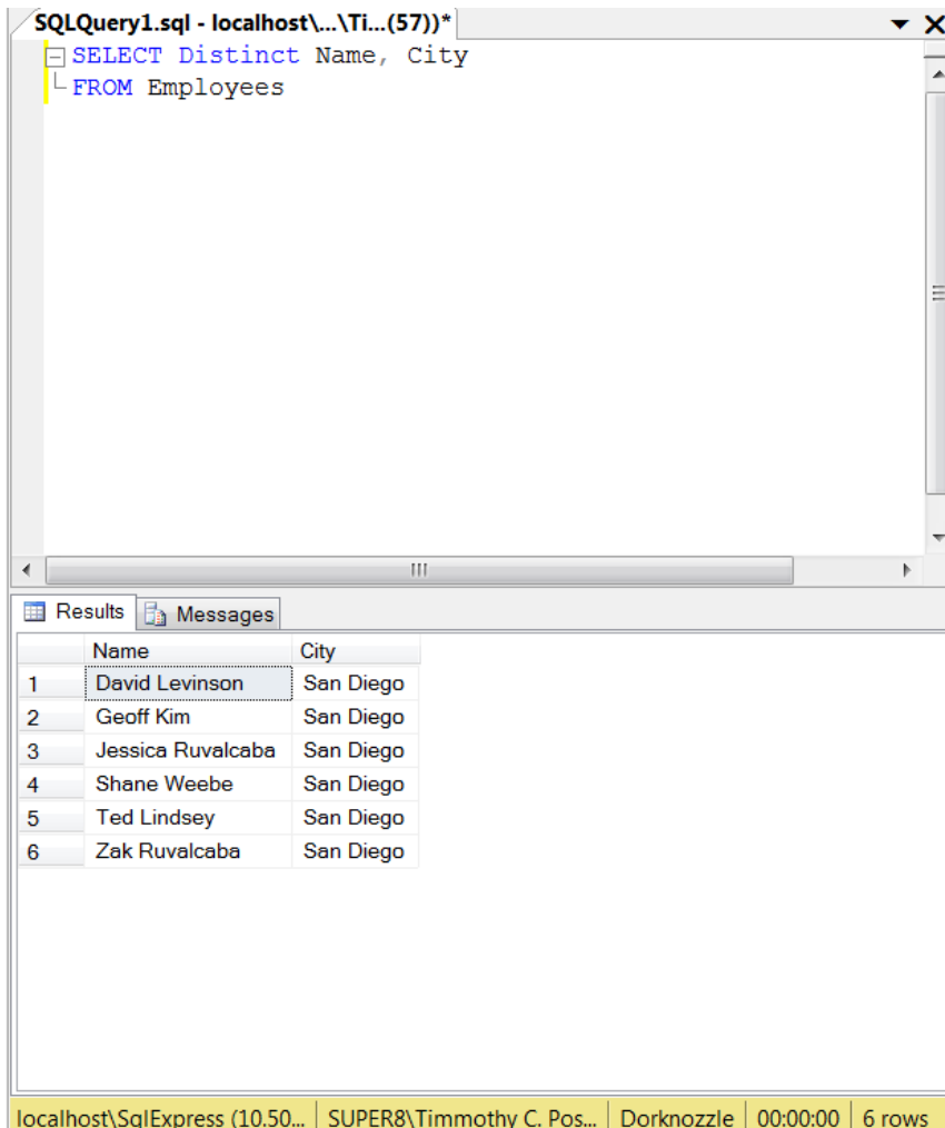
Figure 8.8. Retrieving employees and cities
