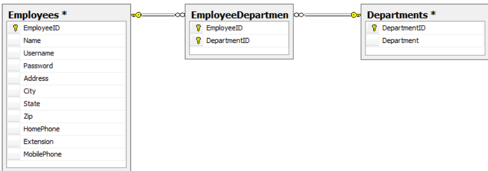
Figure 7.29. Using a mapping table to implement a many-to-many relationship
