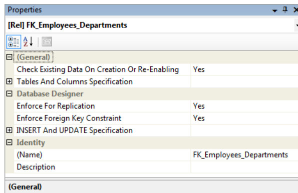
Figure 7.28. The properties of a foreign key
