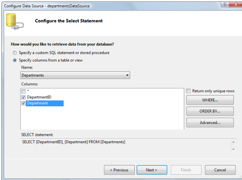
Figure 12.19. Selecting the columns from the Departments table
