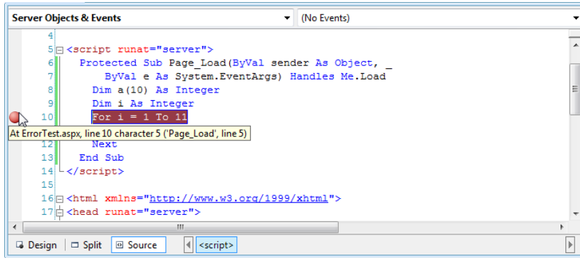
Figure 5.40. Setting a breakpoint
