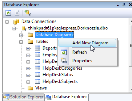
Figure 7.15. Creating a database diagram with Visual Web Developer
