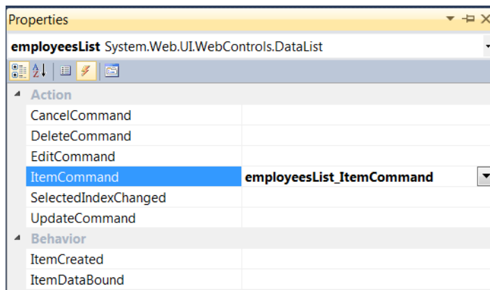
Figure 10.3. The ItemCommand event in the Properties window
