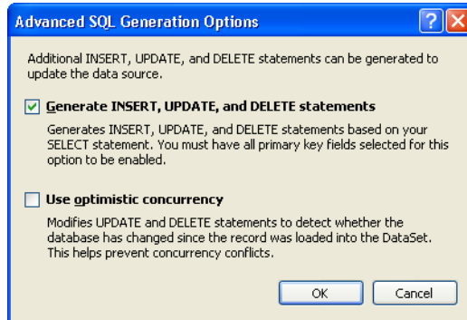
Figure 12.13. Generating INSERT, UPDATE, and DELETE statements
