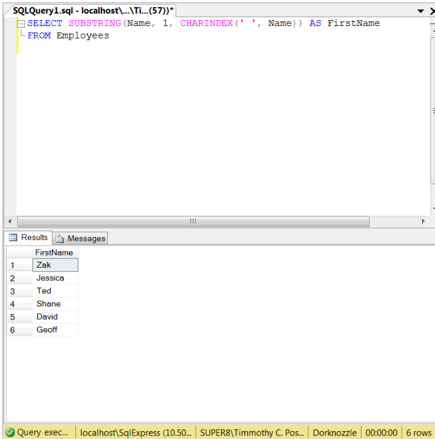
Figure 8.9. Employees' first names
