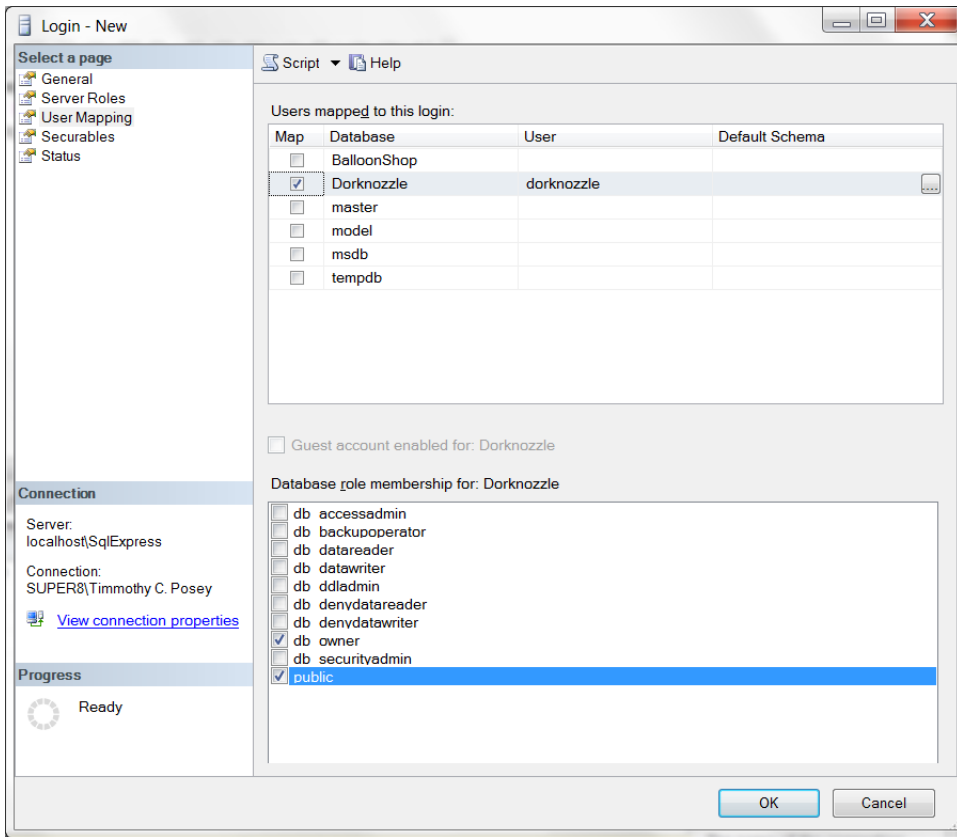
Figure 9.3. Setting the database owner
