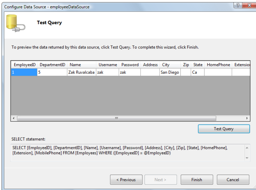
Figure 12.14. Testing the query generated for our data source
