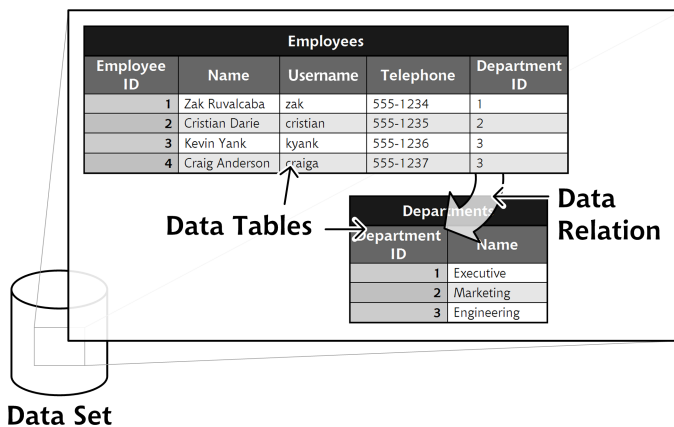
Figure 12.23. The structure of a DataSet , which closely resembles that of a database
