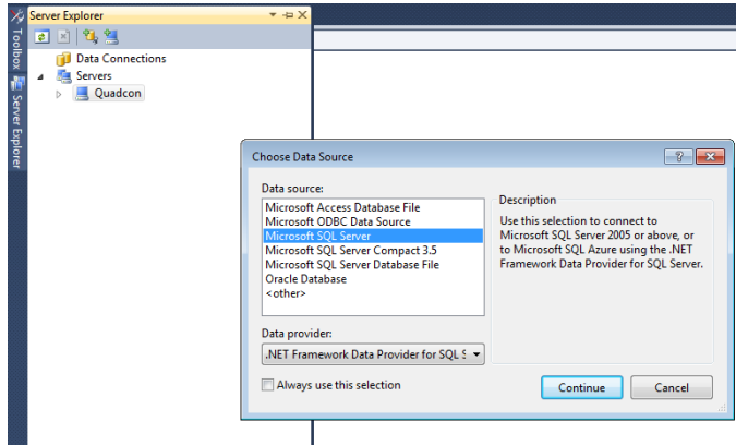
Figure 15.1. Creating a connection with Visual Studio
