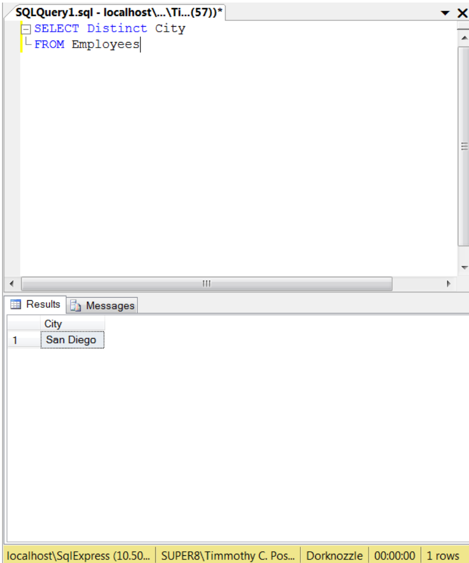
Figure 8.7. Selecting distinct cities
