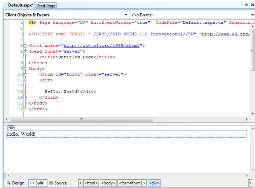
Figure 5.5. Viewing Default.aspx in Web Forms Designer's Source view
