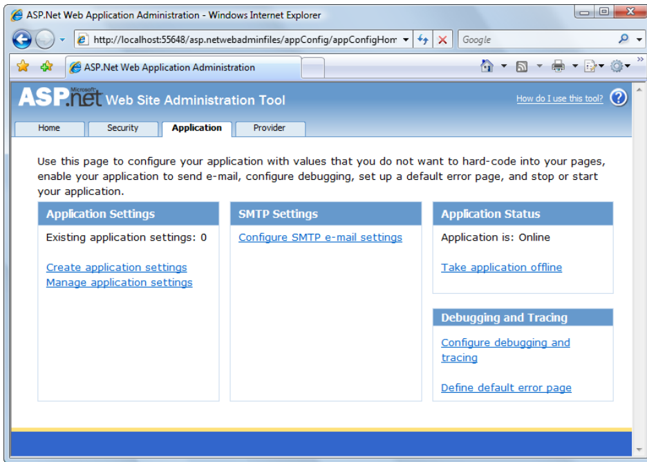
Figure 13.10. Managing application settings
