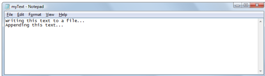
Figure 14.6. Appending text
