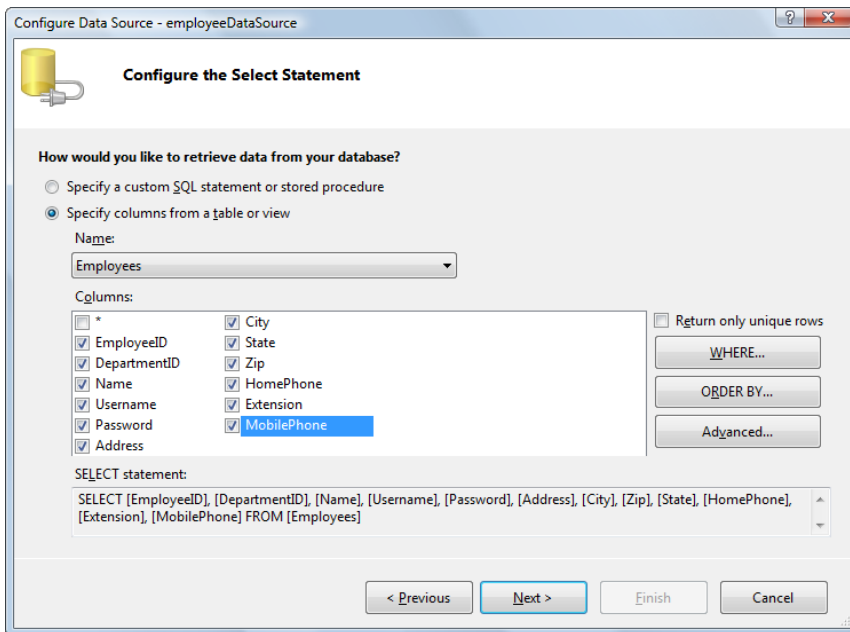
Figure 12.11. Choosing fields
