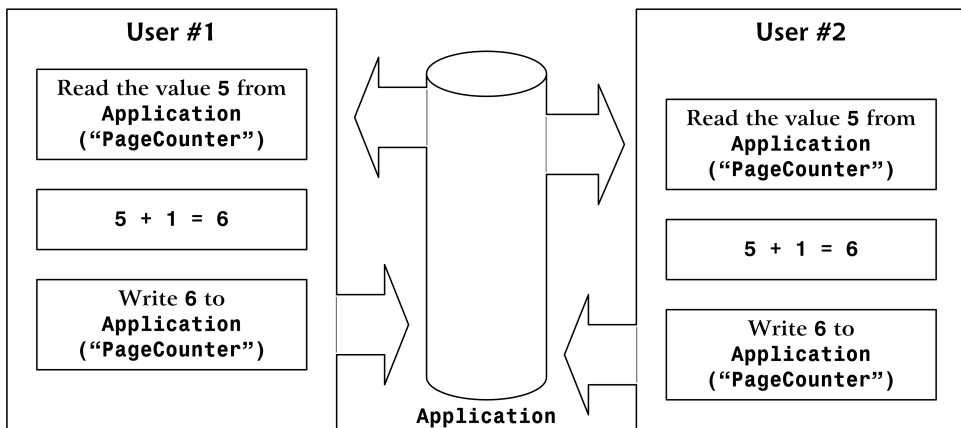
Figure 5.20. Two users updating application state simultaneously
