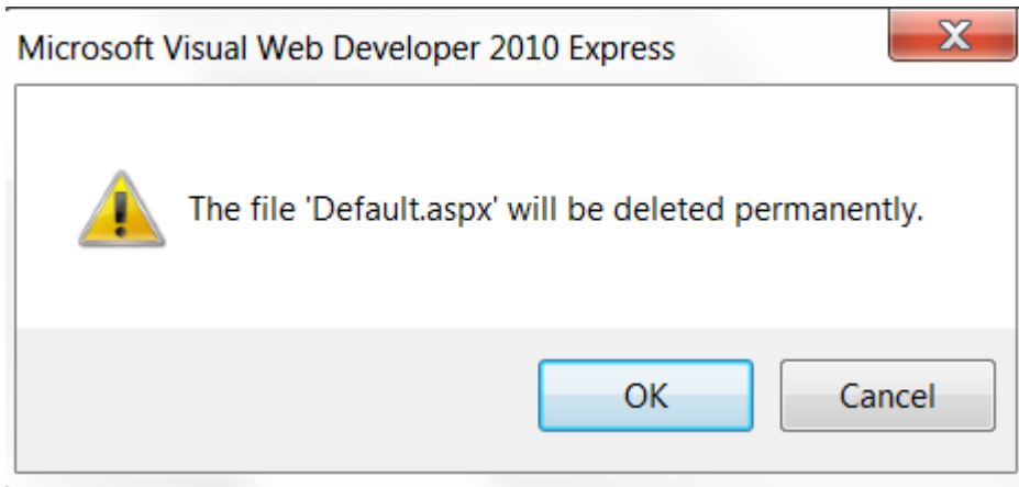
Figure 5.30. Deleting Default.aspx
