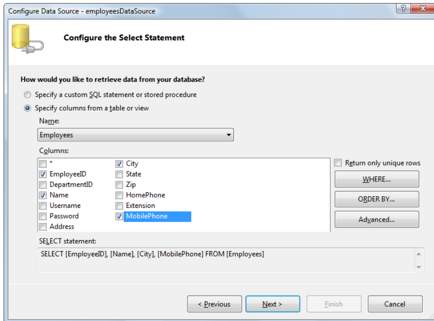
Figure 12.4. Choosing columns
