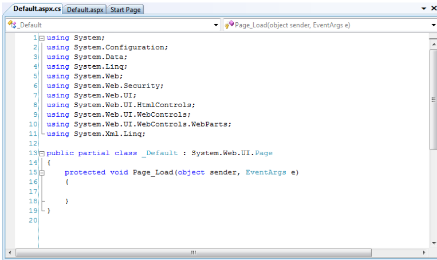
Figure 5.7. Editing Default.aspx.cs
