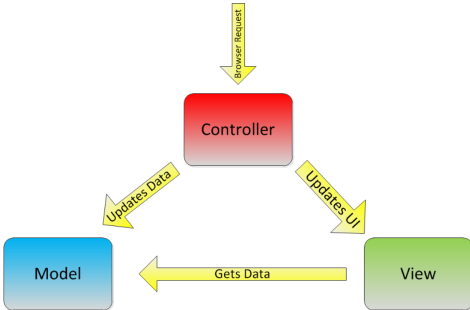
Figure 16.1. Model-View-Controller pattern
