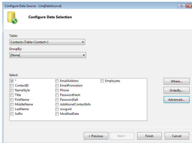
Figure 15.9. Configuring the data selection
