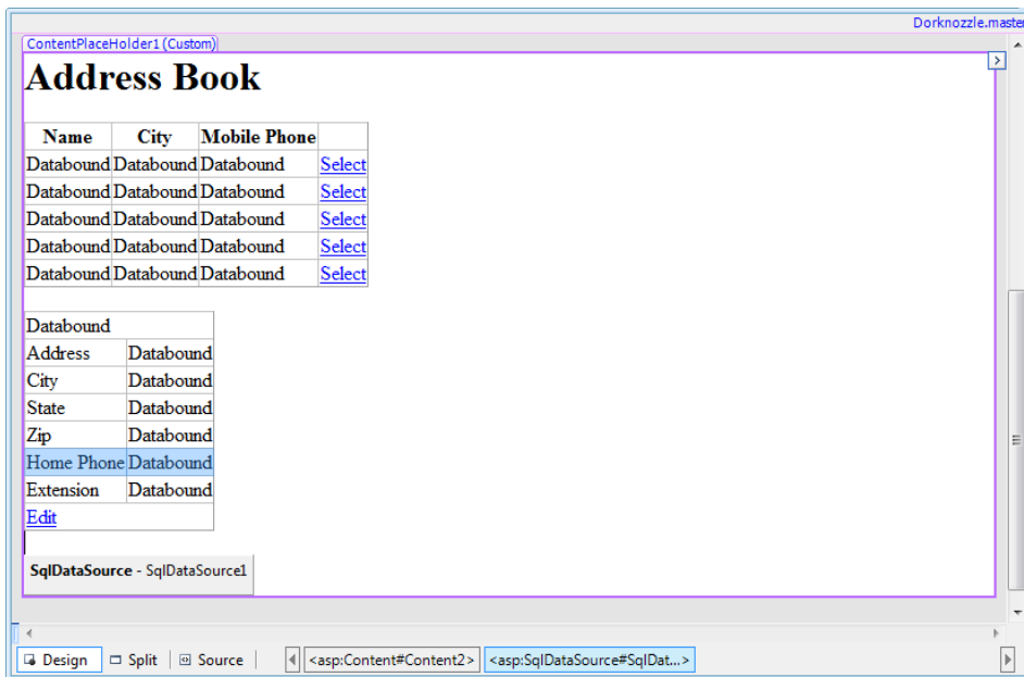
Figure 12.2. AddressBook.aspx with an SqlDataSource control
