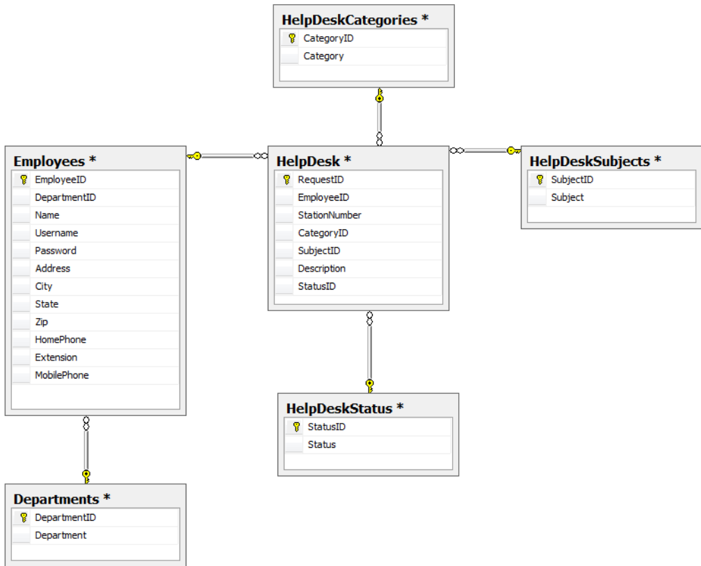
Figure 7.26. Creating and visualizing table relationships
