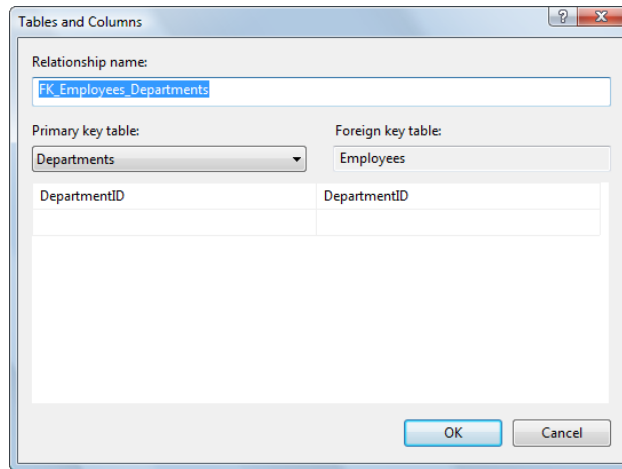
Figure 7.23. Adding a foreign key
