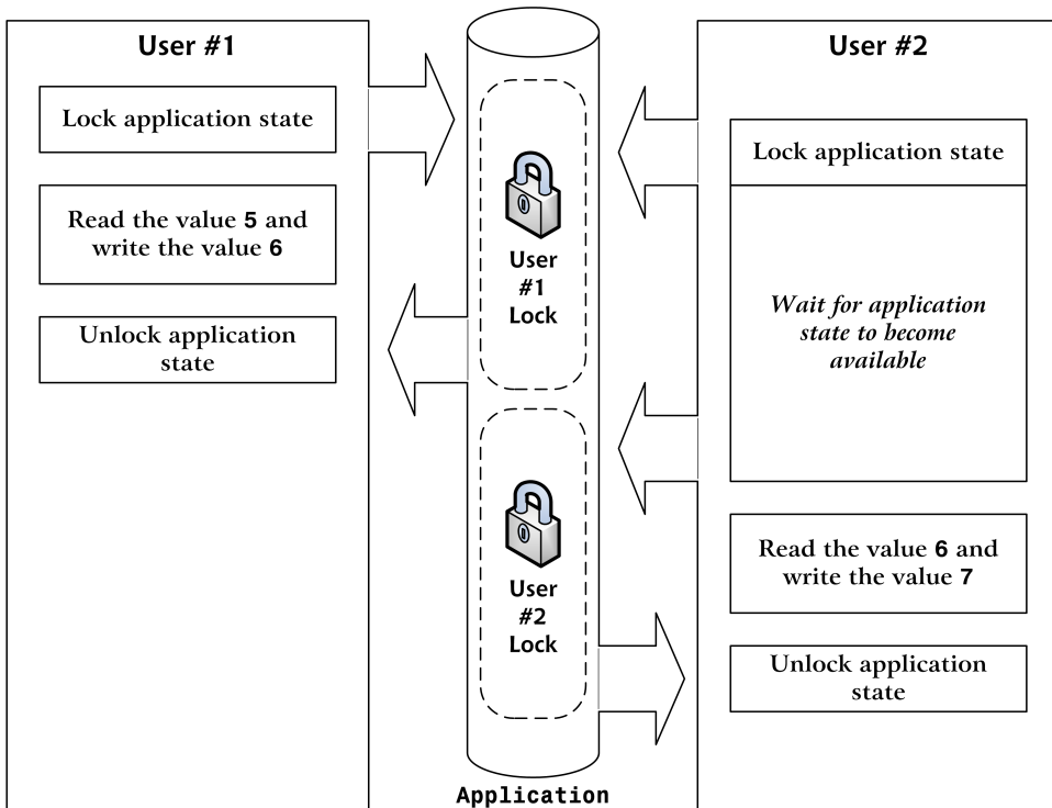
Figure 5.21. Two users updating application state with locks
