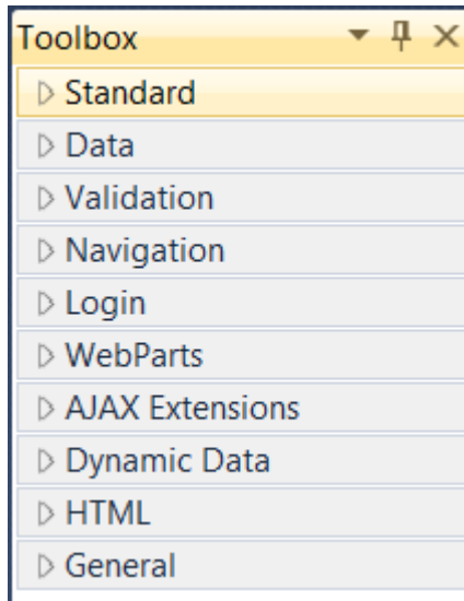
Figure 5.10. The Toolbox
