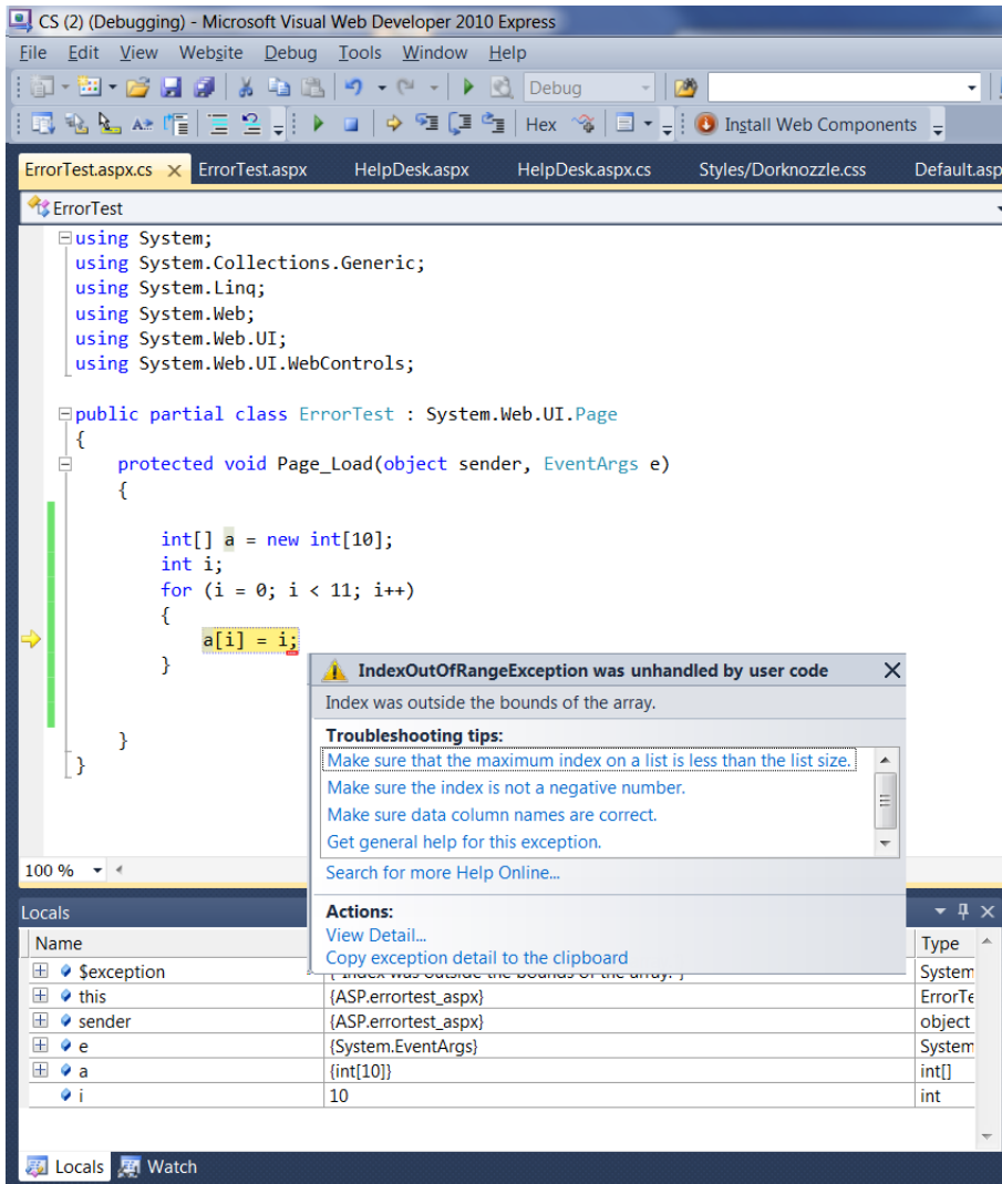
Figure 5.36. Debugging a run-time error
