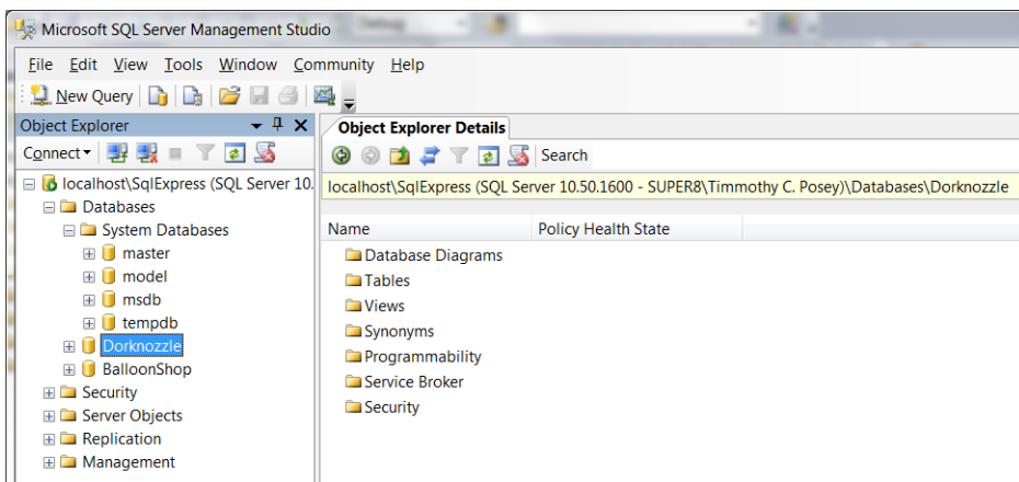
Figure 7.5. Inspecting your SQL server instance
