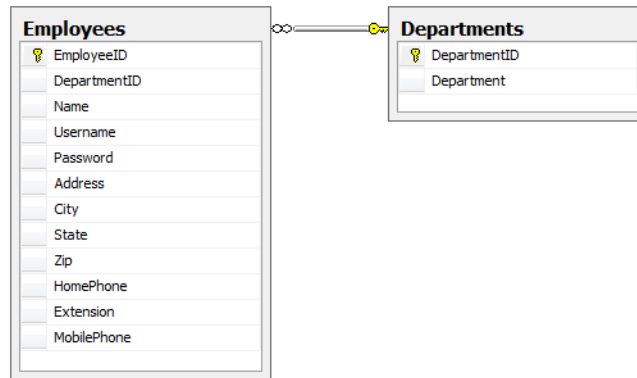
Figure 7.27. Database diagram showing a one-to-many relationship
