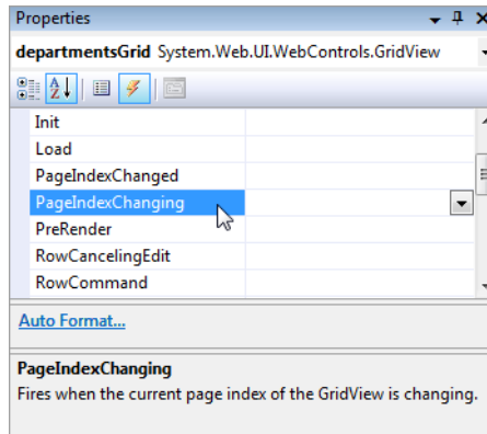
Figure 12.26. Creating the PageIndexChanging event handler
