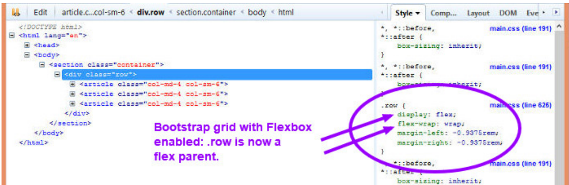
Bootstrap flex element
