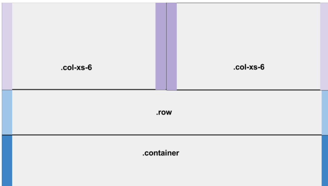
Bootstrap columns with padding
