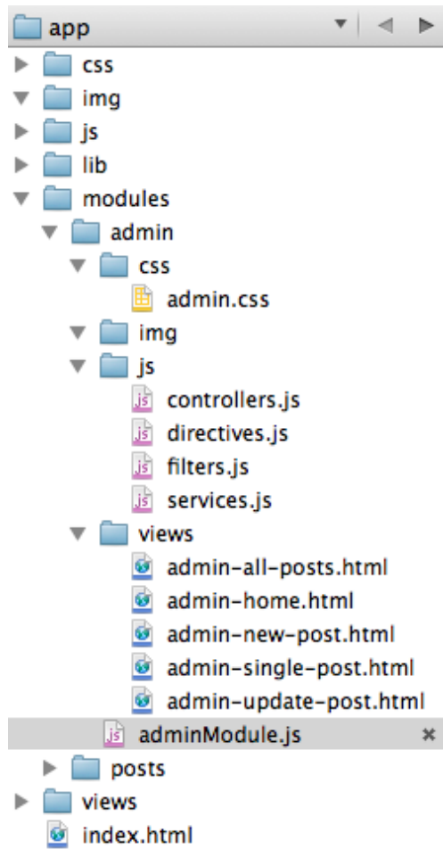
Figure 7.1. Admin Module Structure
