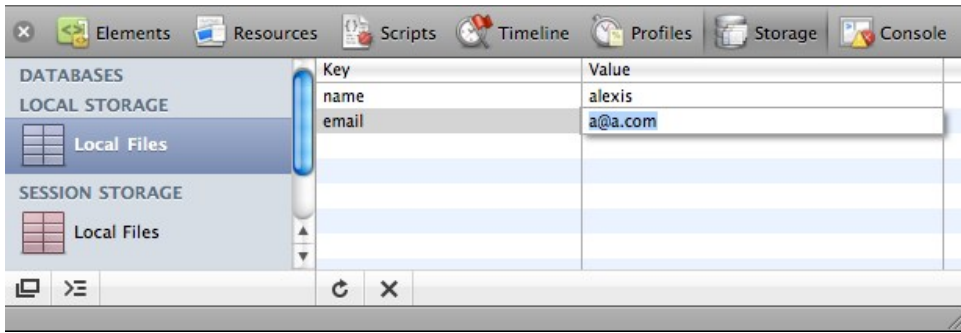
Figure 11.7. Modifying the values stored in Web Storage
